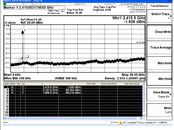
802.11b-Low channel
