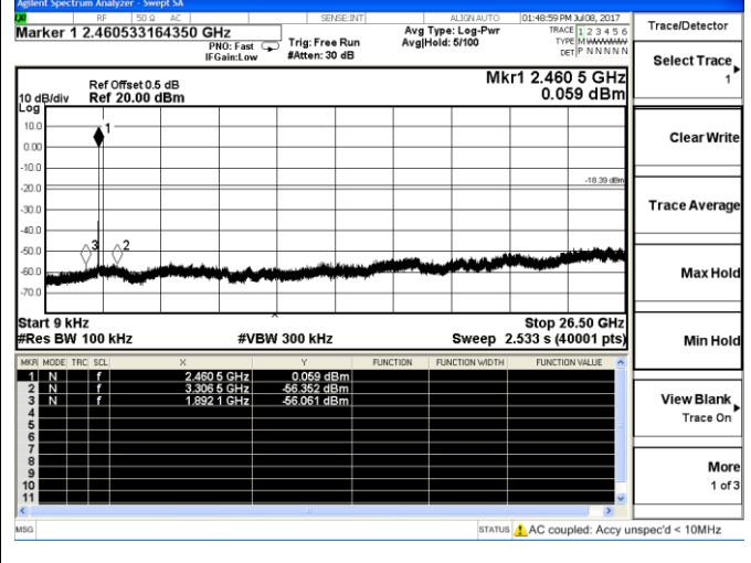
802.11b-High channel
