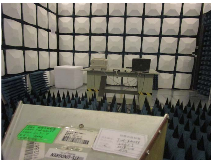
Radiated Emission Rear View (Downloading Above 1GHz)
