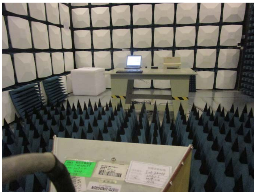
Radiated Emission Front View (Downloading Above 1GHz)
