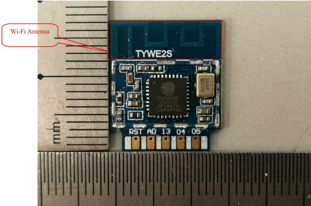
EUT – PCB Chip View
