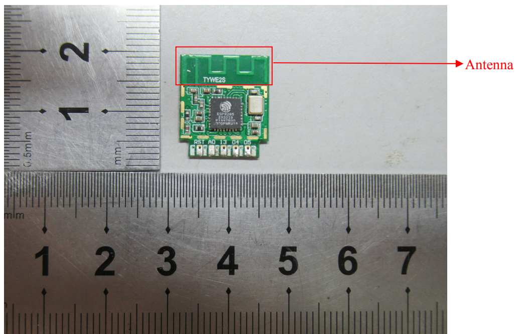
EUT – PCB-2 Top View
