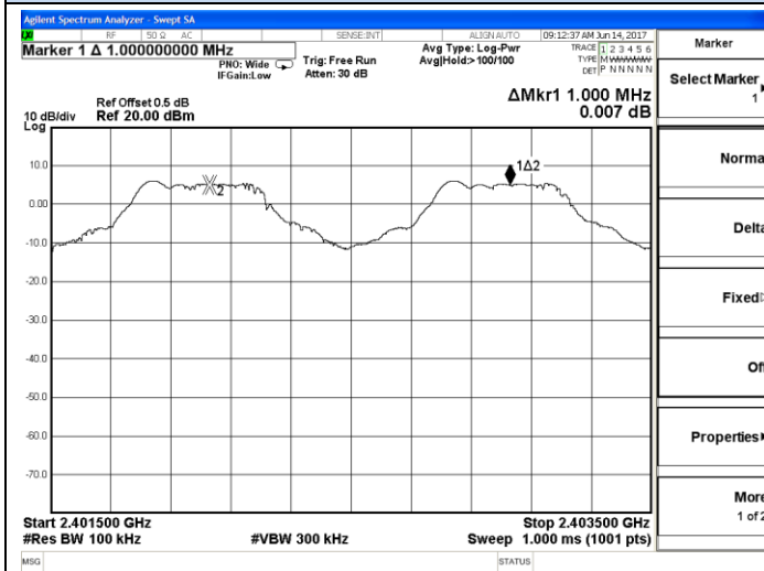
Channel 0 / 2402 MHz
