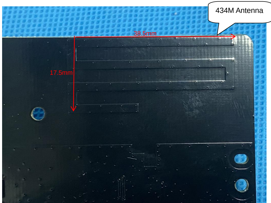
INTERNAL VIEW OF EUT (FIGURE 8)
