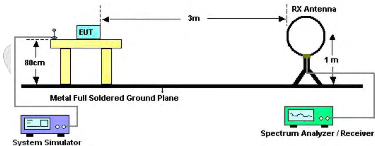
Figure 1. Below 30MHz
