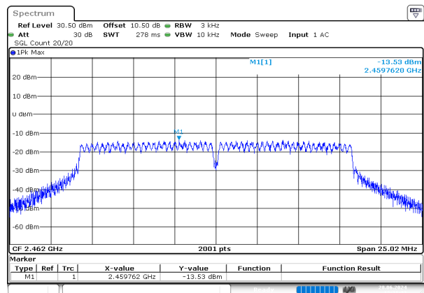
g_2462MHz_Chain 0
