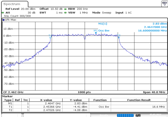
g_2462MHz_Chain 0
