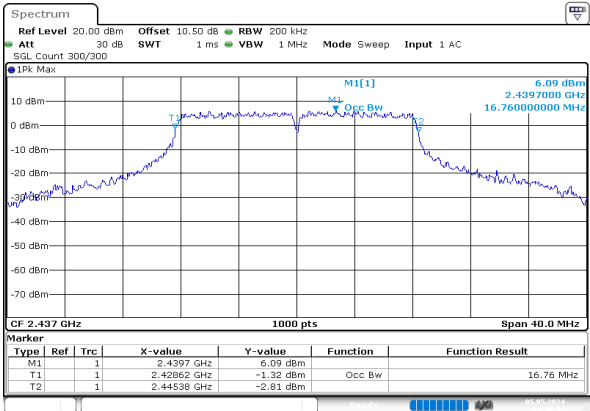
g_2437MHz_Chain 0
