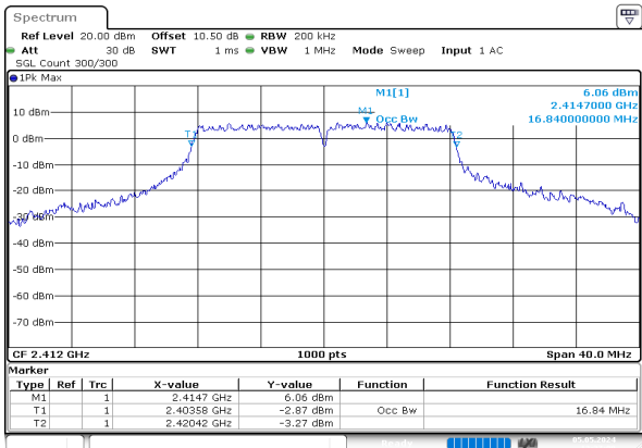
g_2412MHz_Chain 0
