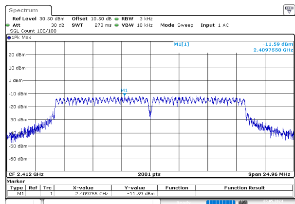
g_2412MHz_Chain 0
