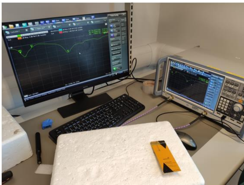
VNA Setup
