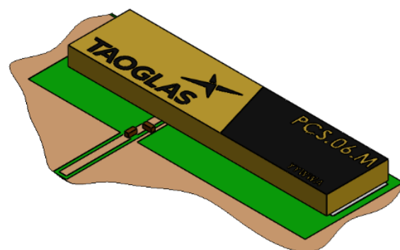
ANTENNA ON FOOTPRINT PCB VIEW SCALE 3:1
