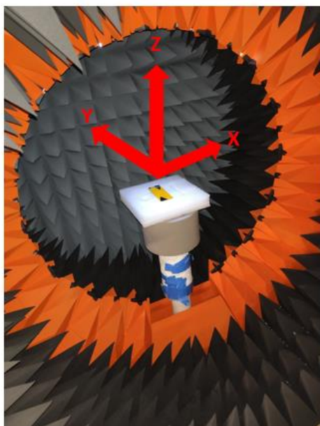
Chamber Setup
