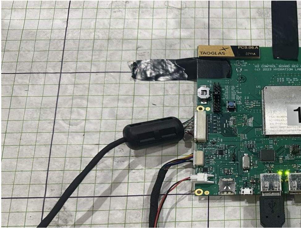
Modification made during 2.4GHz testing : Ferrite 0431164951 on LVDS cable on sample 11
