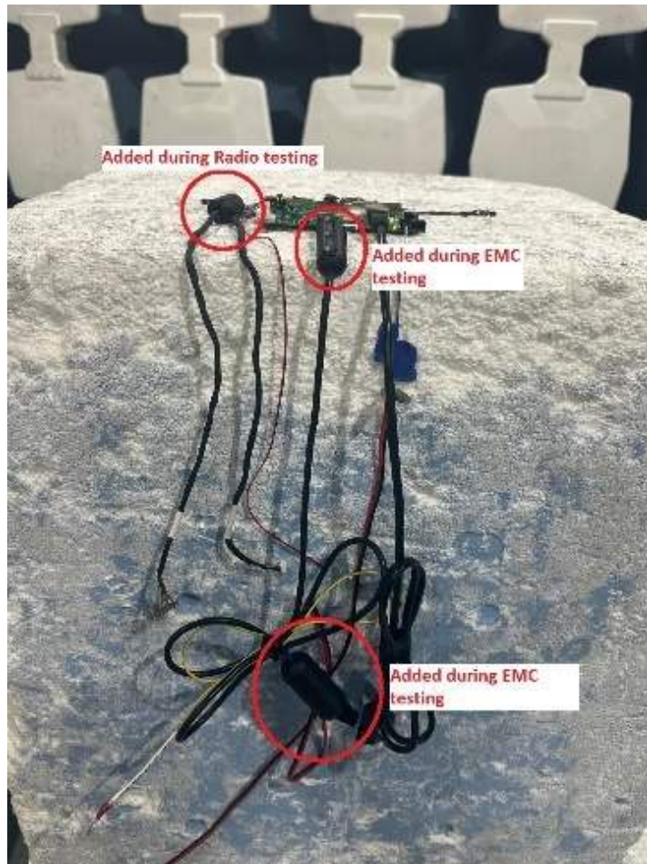
Overall EUT modification state during EMC & 5GHz Wireless testing
