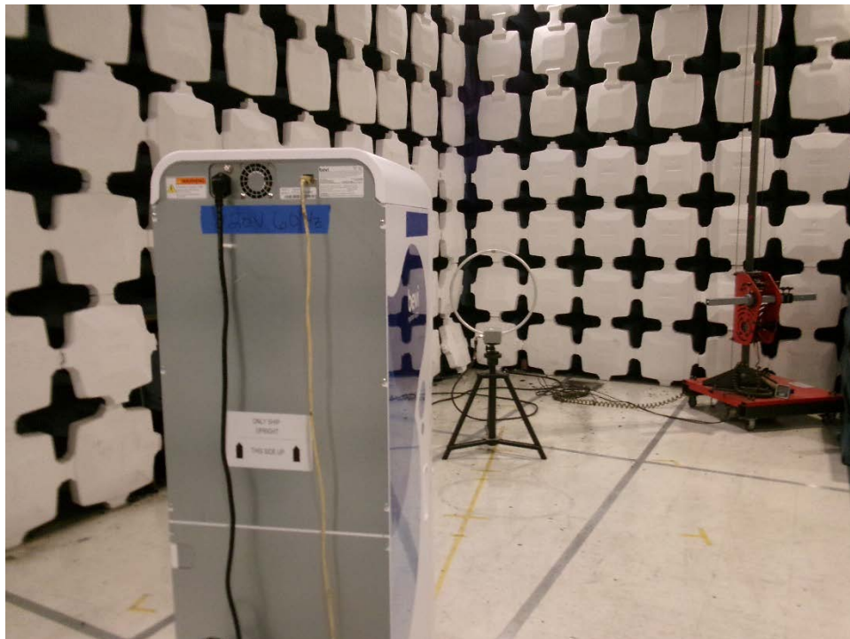
Parallel Rear
