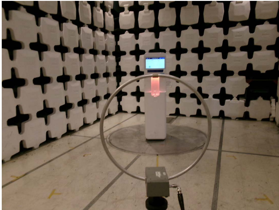
Parallel Front
