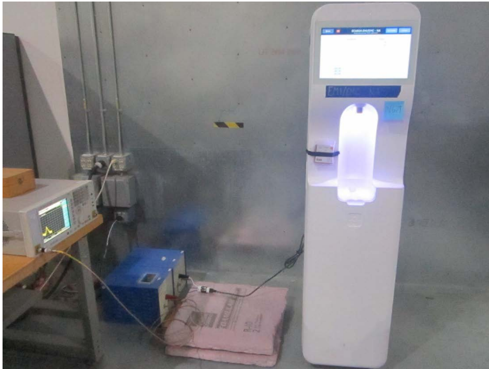
AC line conducted testing Front
