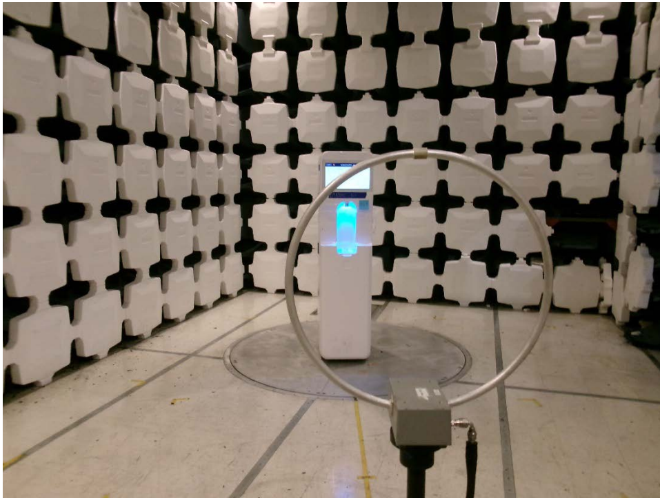
9k-30MHz Front
