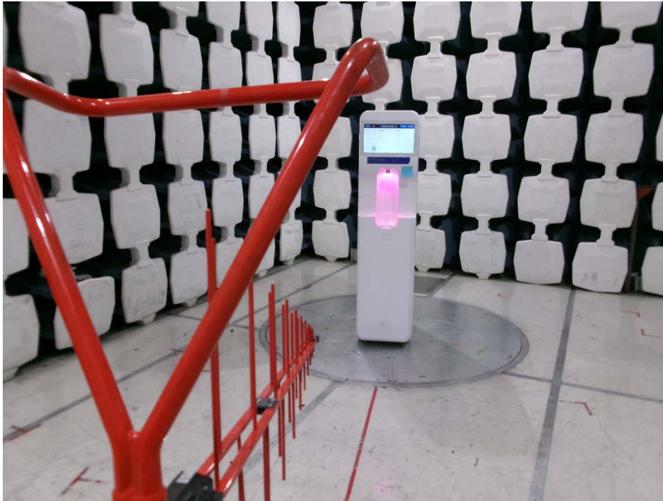
30MHz-1GHz Front
