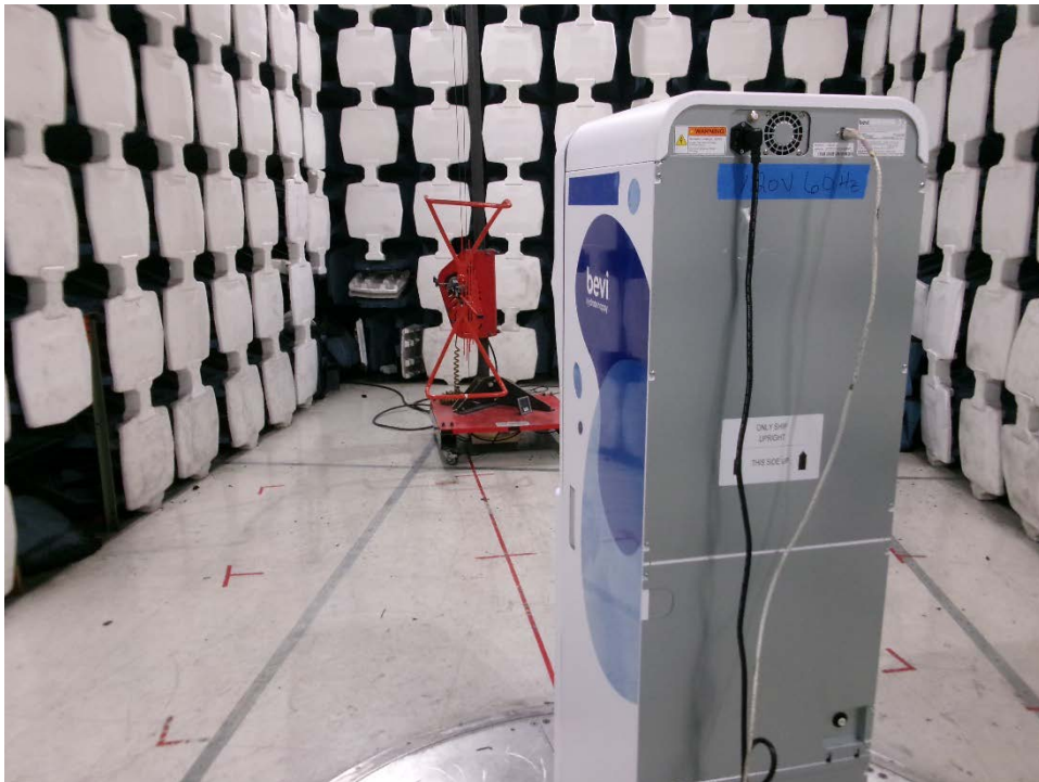
30MHz-1GHz Rear
