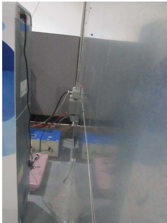
AC line conducted testing Rear
