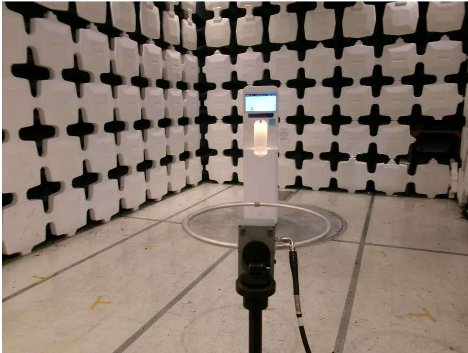
Parallel to the ground Front
