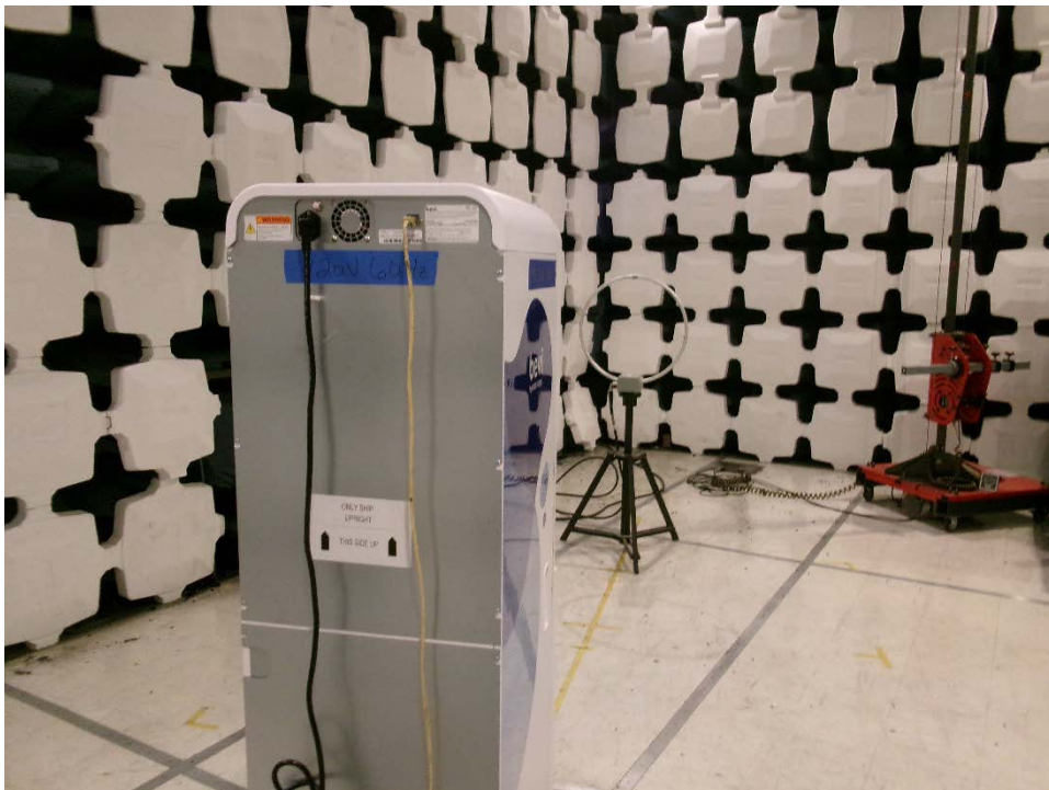
9k-30MHz Rear
