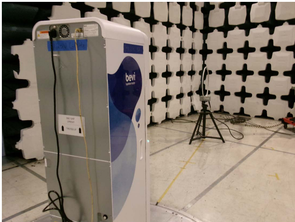
Perpendicular Rear
