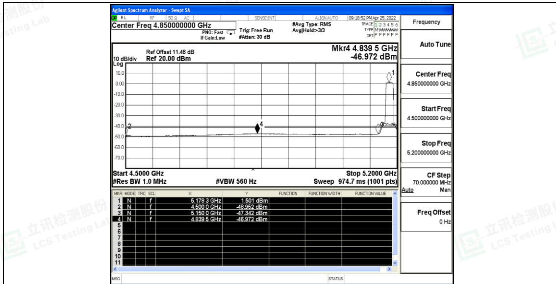
11N20SISO_Ant_Low_5180_Peak
