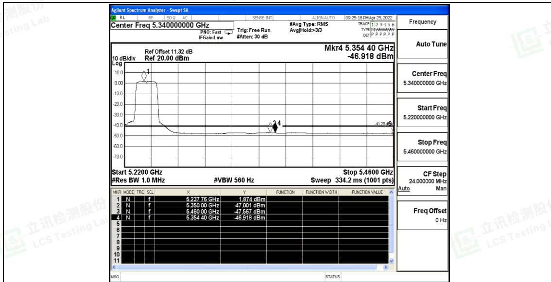
11N20SISO_Ant_High_5240_Peak
