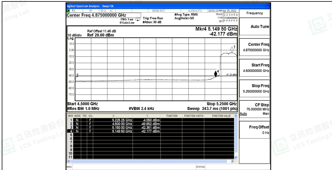
11AC80SISO_Ant_Low_5210_Peak
