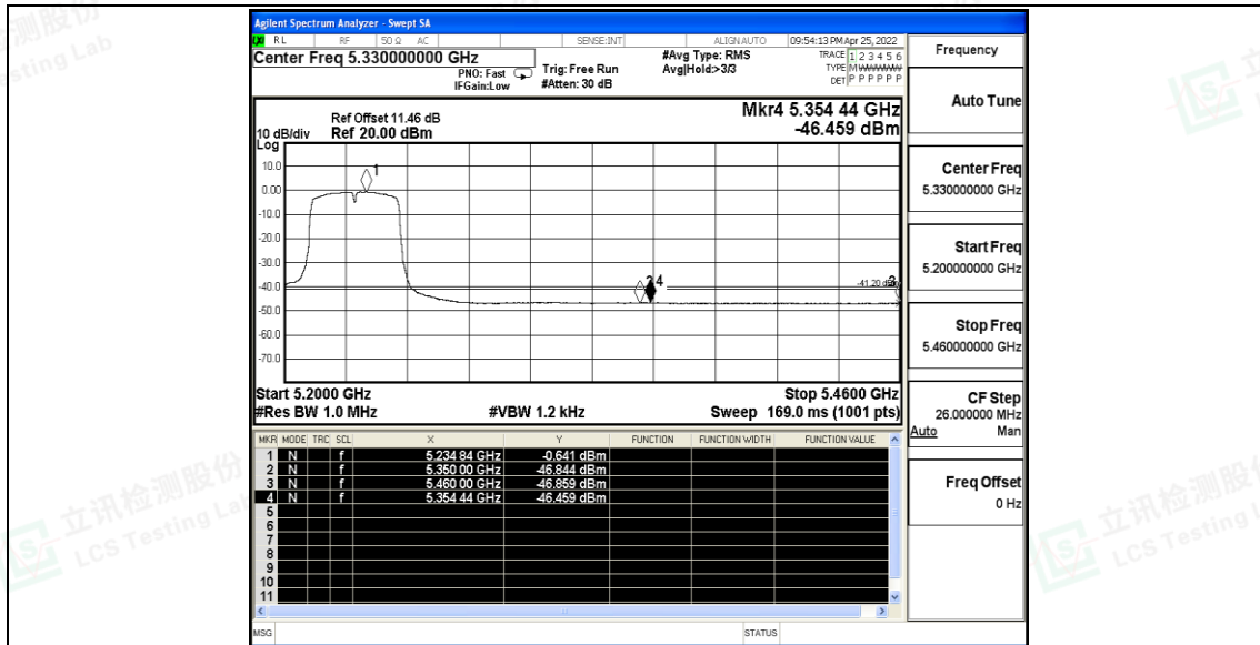
11AC40SISO_Ant_High_5230_Peak
