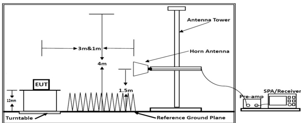
Above 1GHz
