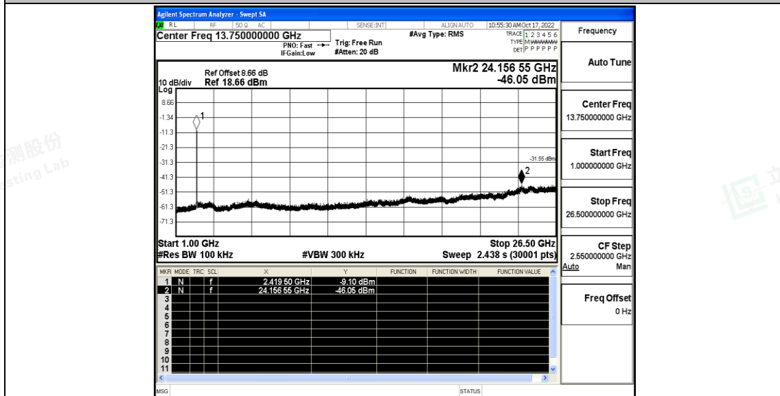
11N40SISO_Ant_2437_0~Reference
