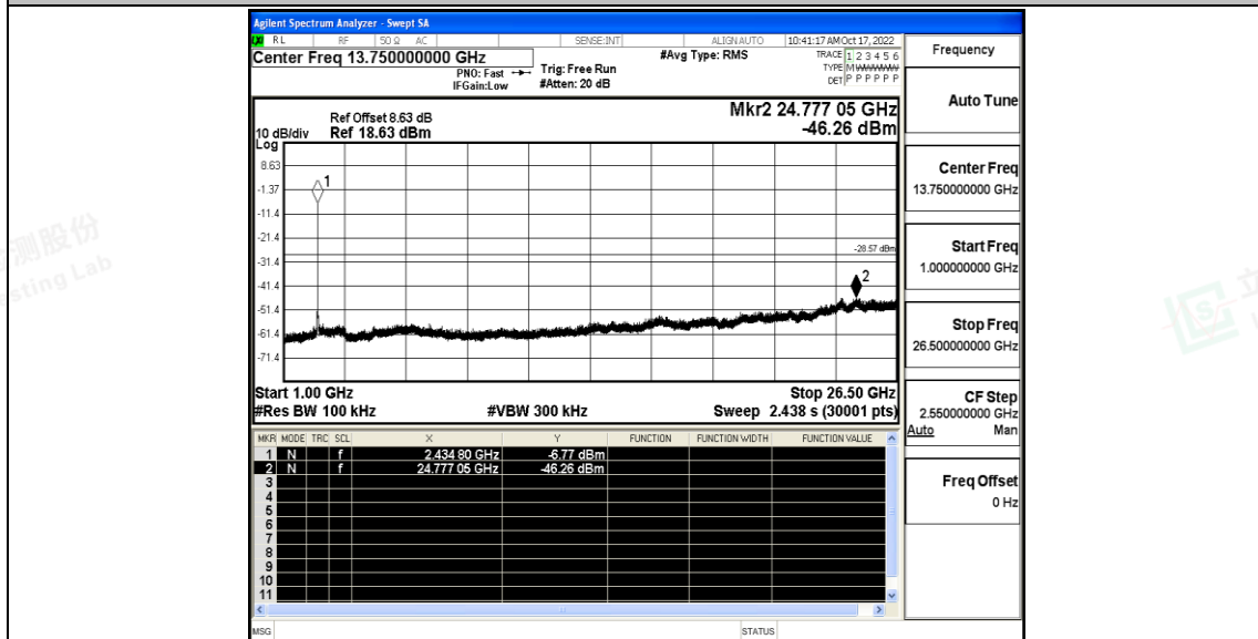
11N20SISO_Ant_2462_0~Reference
