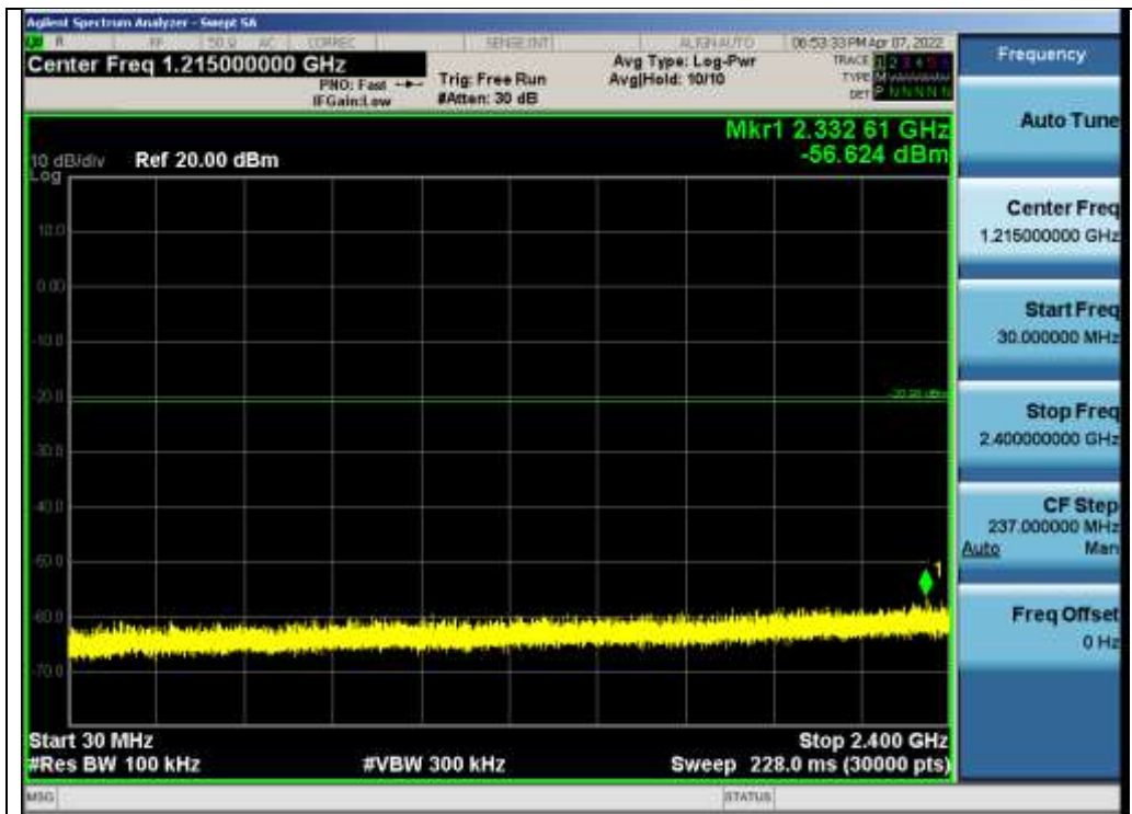
Test_Graph_LE1M_ANT1_2430_1Mbps_Lower Band Emissions
