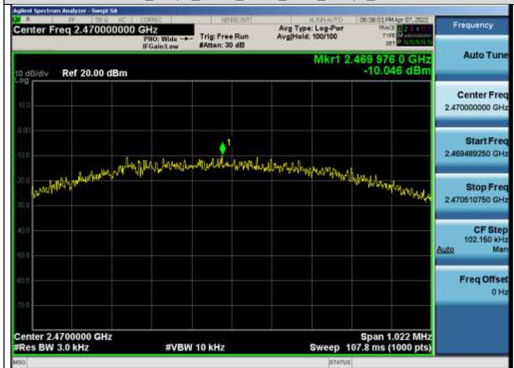
Test_Graph_LE1M_ANT1_2470_1Mbps_PSD
