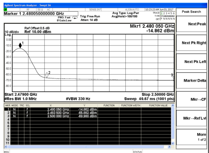
Channel 4 / 2480 MHz – Average
