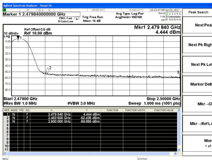
Channel 4 / 2480 MHz – Peak
