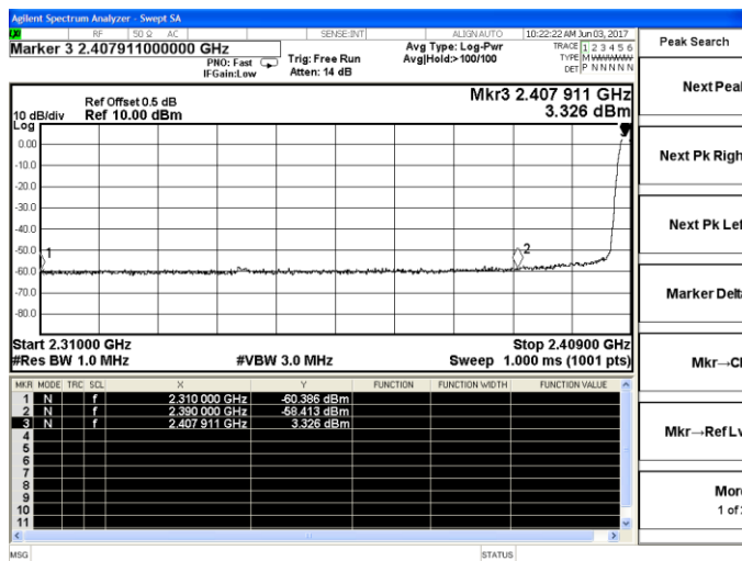
Channel 1 / 2408 MHz – Peak
