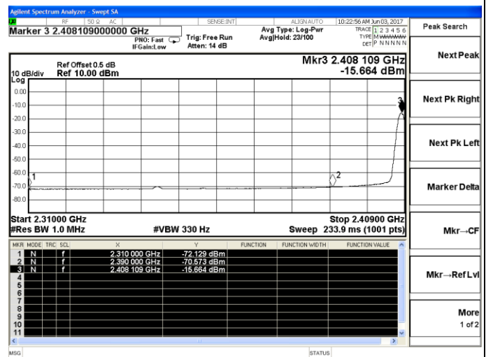
Channel 1 / 2408 MHz – Average
