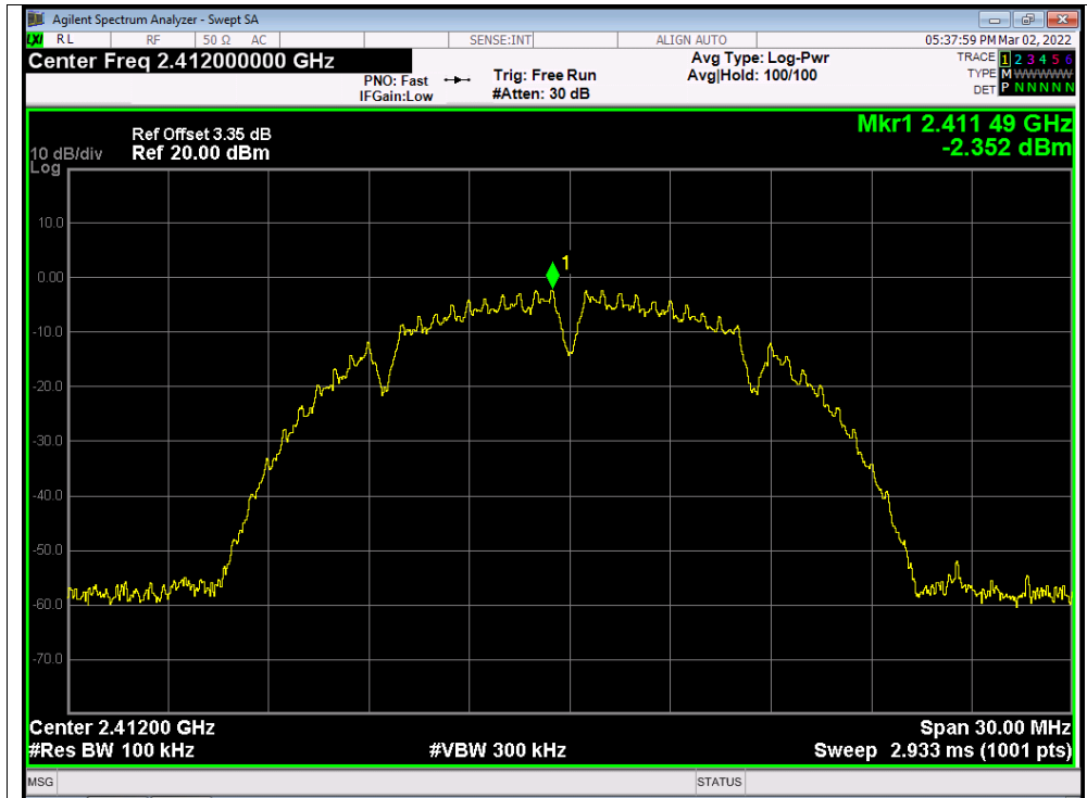
Tx. Spurious NVNT b 2412MHz Emission
