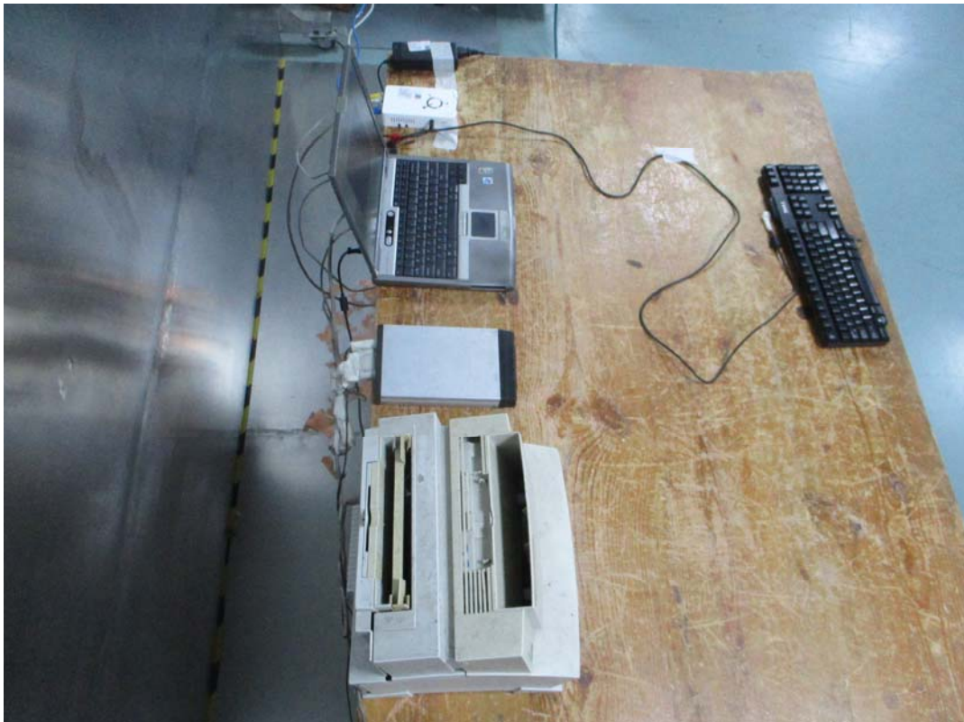
Conducted Emissions Side View- AC/DC Adapter
