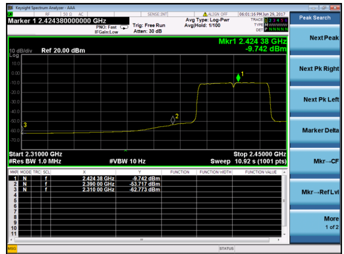
802.11n-HT40-Low channel(Average)
