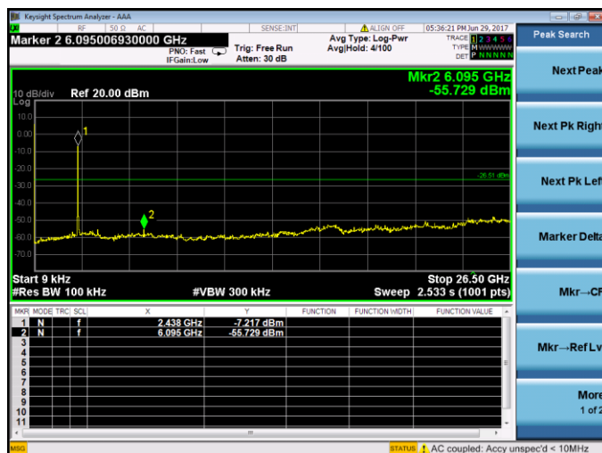
802.11g-Middle channel
