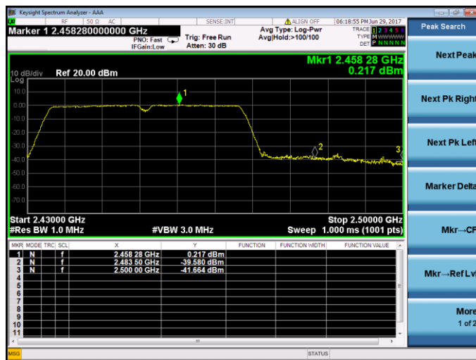
802.11n-HT40-High channel(Peak)
