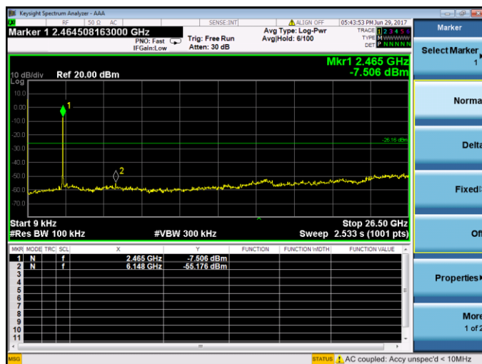
802.11n-HT20-High channel
