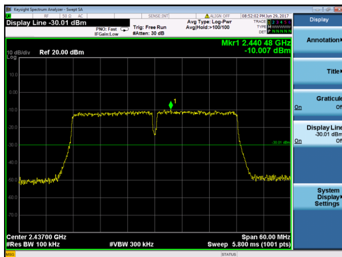
IEEE 802.11n HT40-Channel 6 / 2437 MHz
