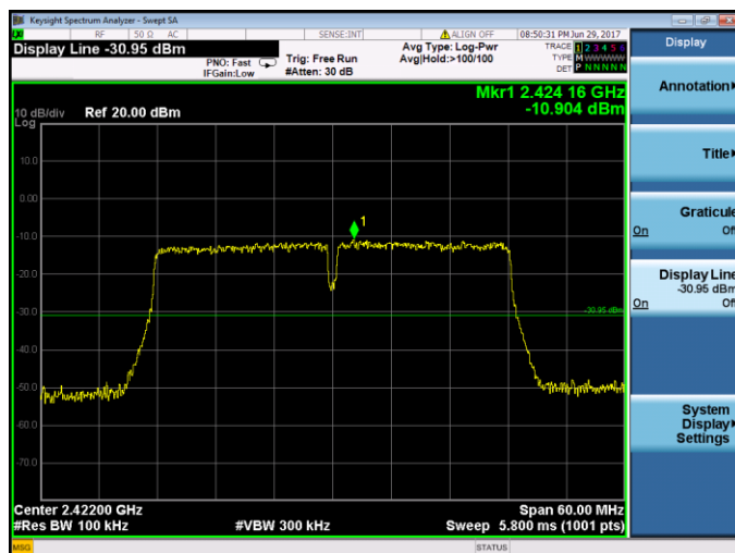
IEEE 802.11n HT40-Channel 3 / 2422 MHz
