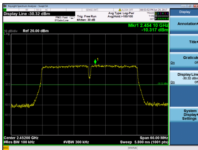
IEEE 802.11n HT40-Channel 9 / 2452 MHz
