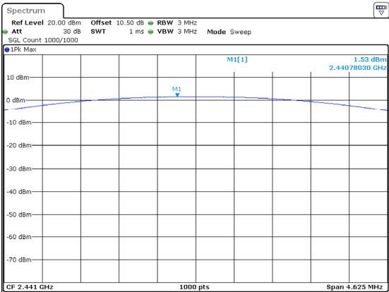
DH1_Middle 1.53dBm
