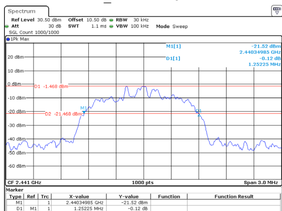
2DH1_Middle 1.252MHz
