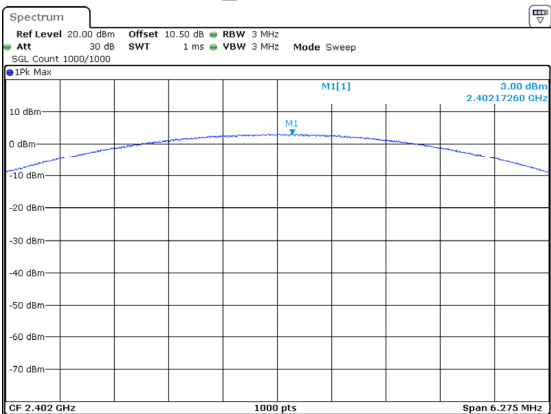
2DH1_Low 3.00dBm
