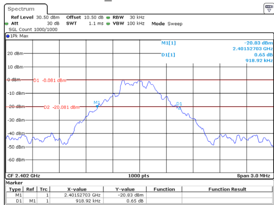
DH1_Low 0.919MHz
