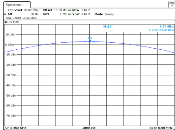
3DH1_Low 3.25dBm
