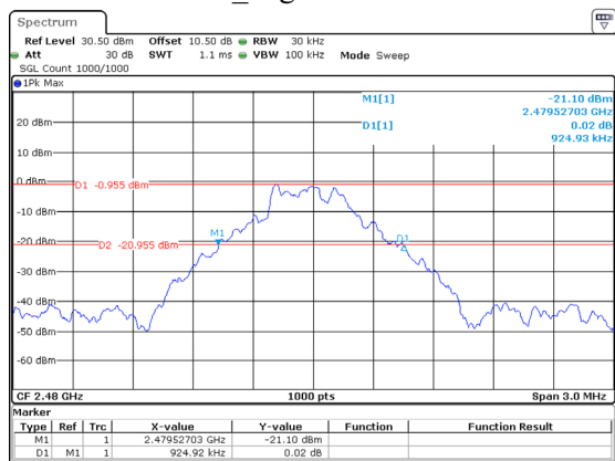
DH1_High 0.925MHz
