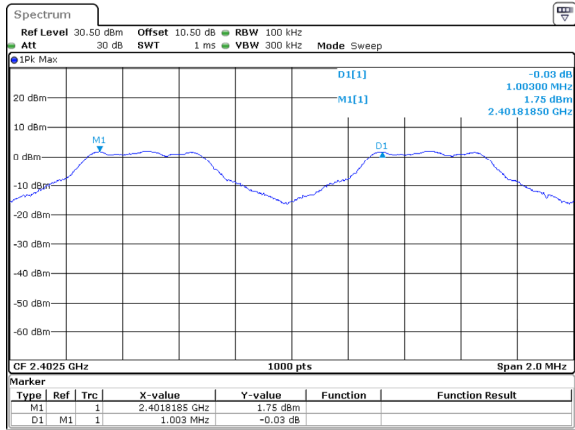
DH1_Low 1.003MHz
