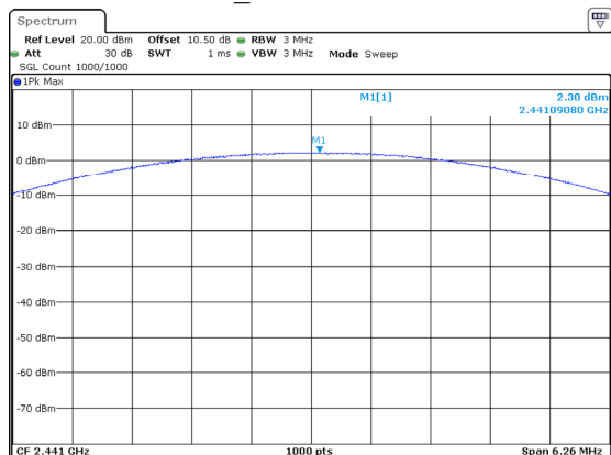
2DH1_Middle 2.30dBm
