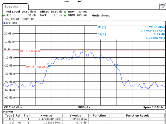
2DH1_High 1.252MHz
