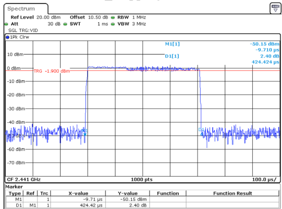
2DH1_Hopping 0.424ms
