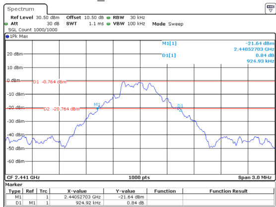
DH1_Middle 0.925MHz
