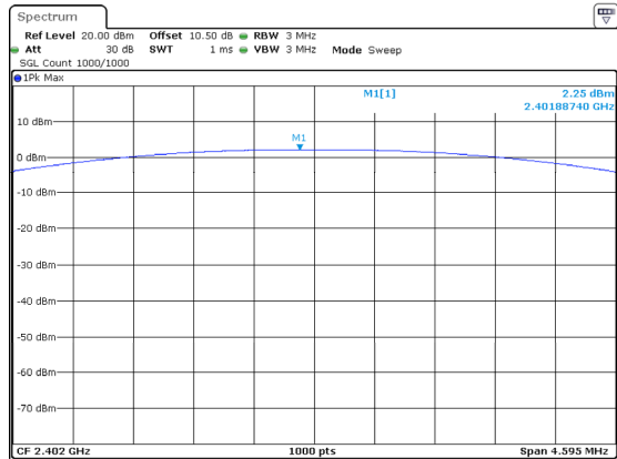
DH1_Low 2.25dBm
