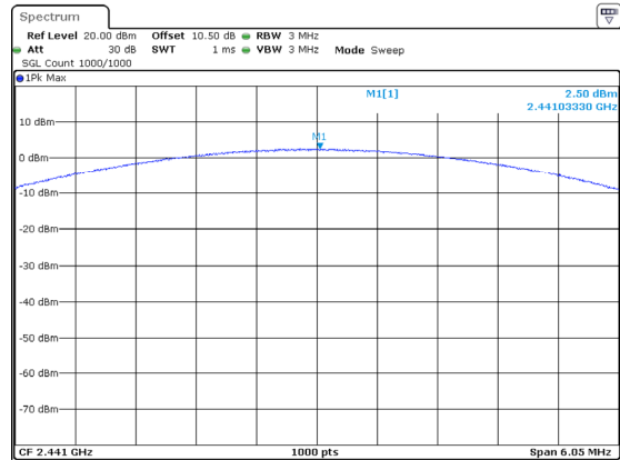
3DH1_Middle 2.50dBm
