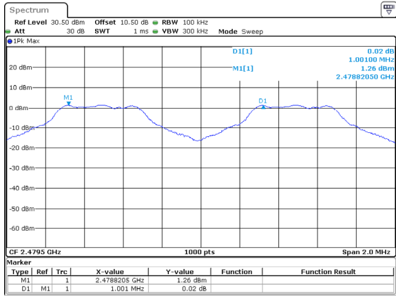
DH1_High 1.001MHz
