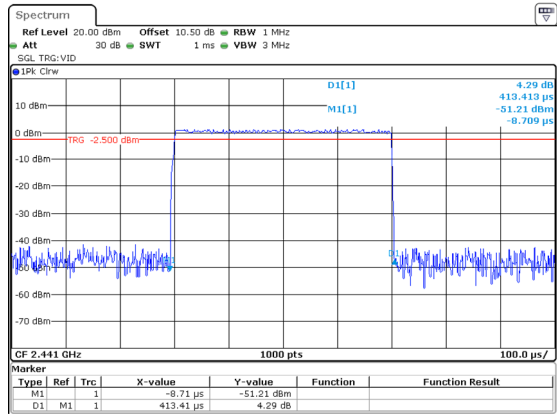
DH1_Hopping 0.413ms
