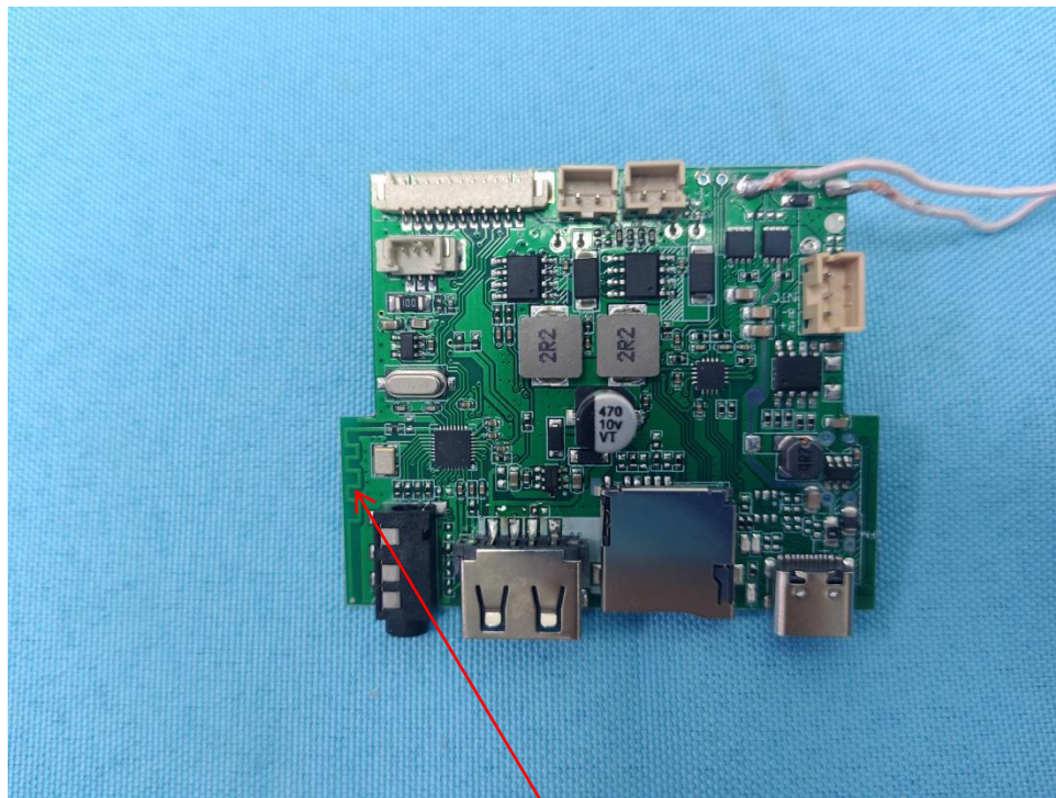
BT-ANT
