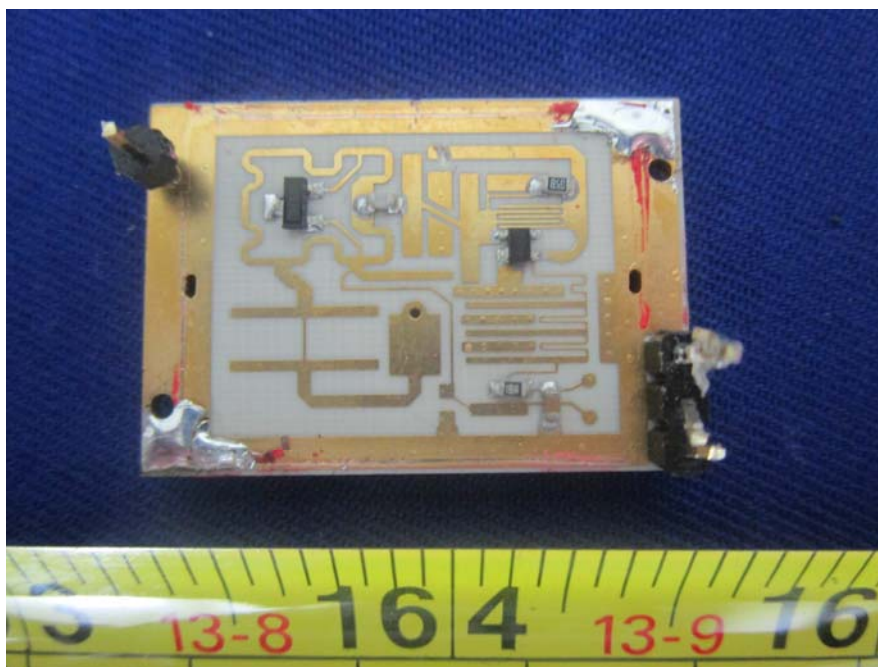
EUT – RF Chip&ANT View
