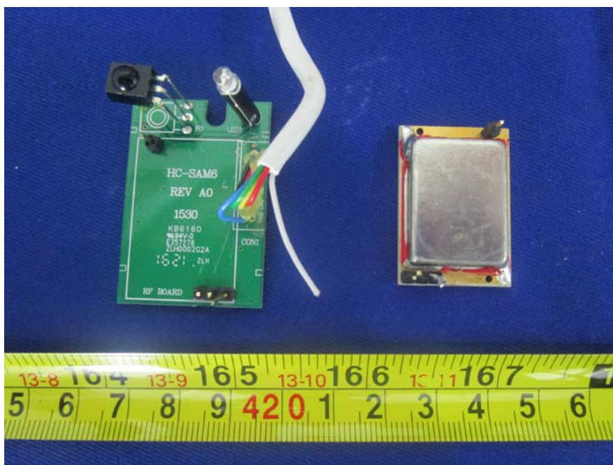
EUT –Sensor Board uncover View
