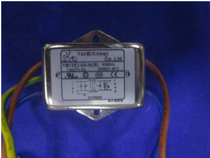
EUT –Filter Label View
