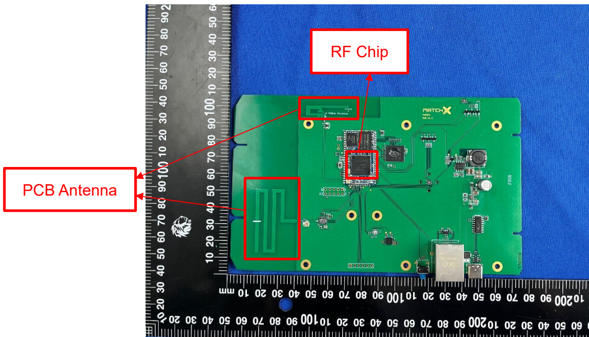
MAIN BOARD TOP VIEW (WITHOUT SHIELDING)
