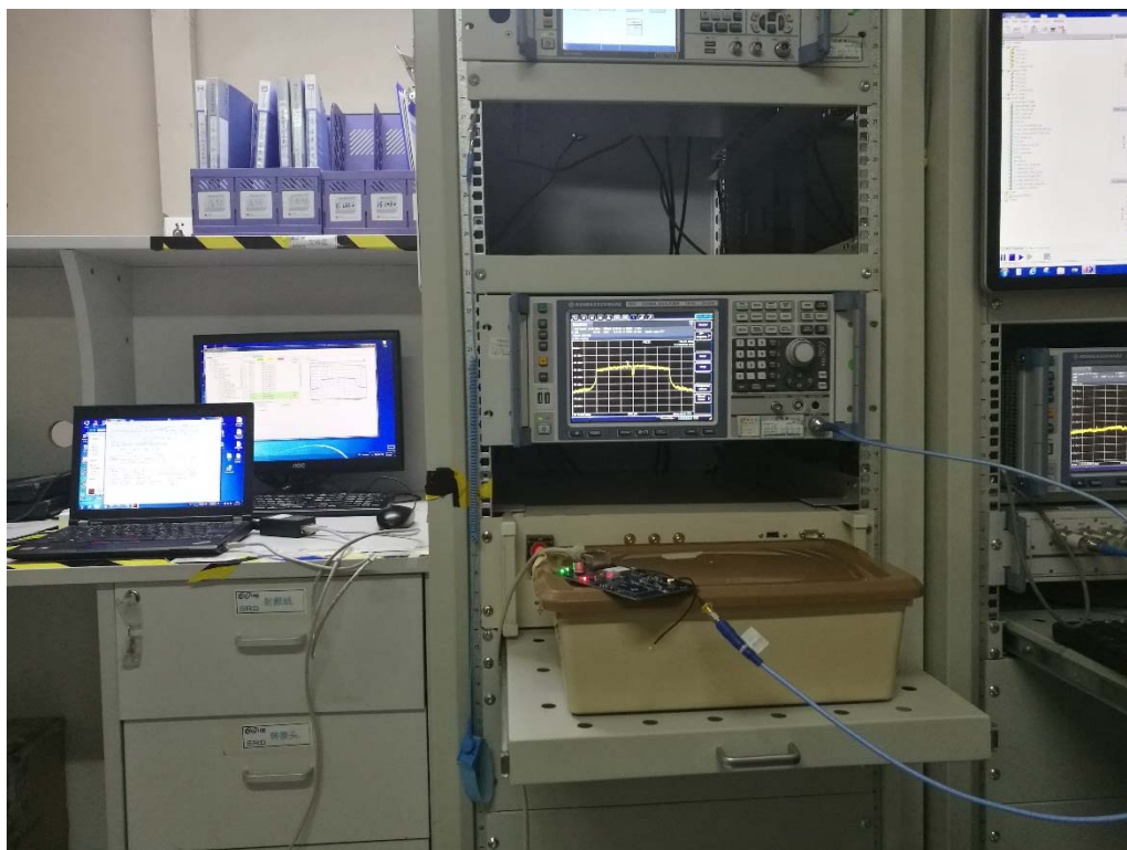
Conducted Test 1
