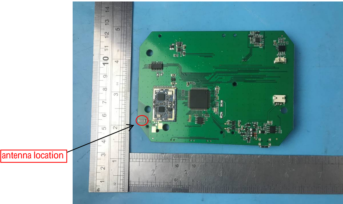
INTERNAL PHOTO OF SAMPLE – 6
