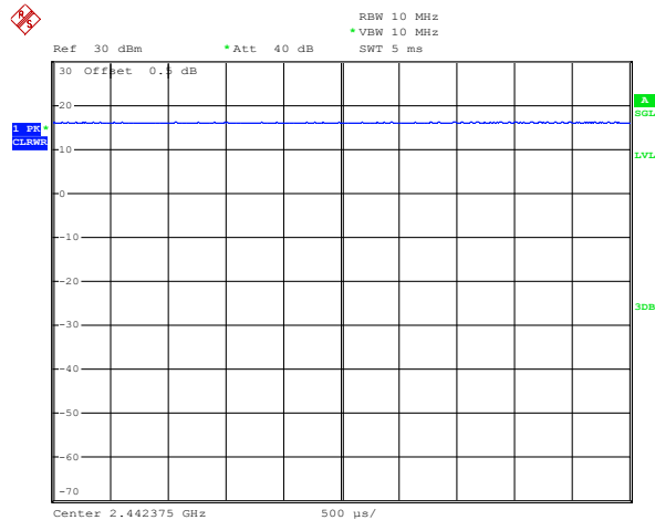
Channel 10 / 2442.375 MHz
