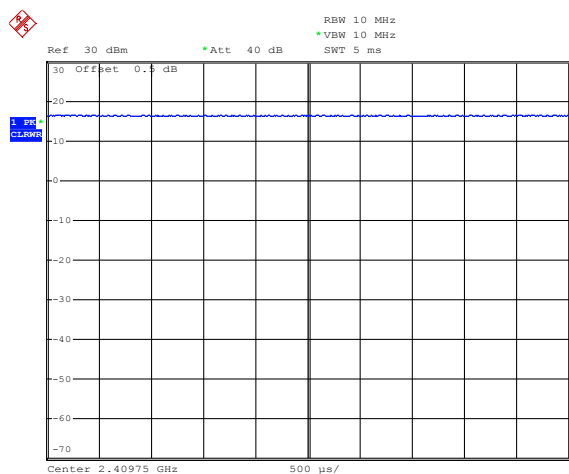
Channel 1 / 2409.750 MHz
