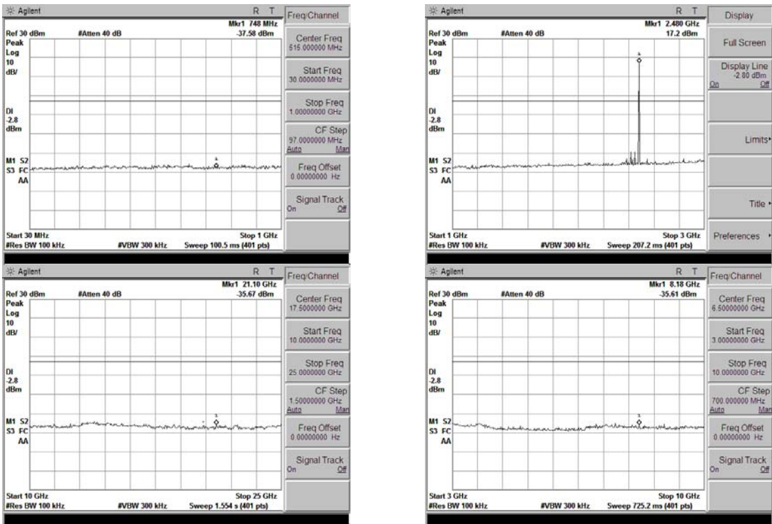
GFSK Mode,
