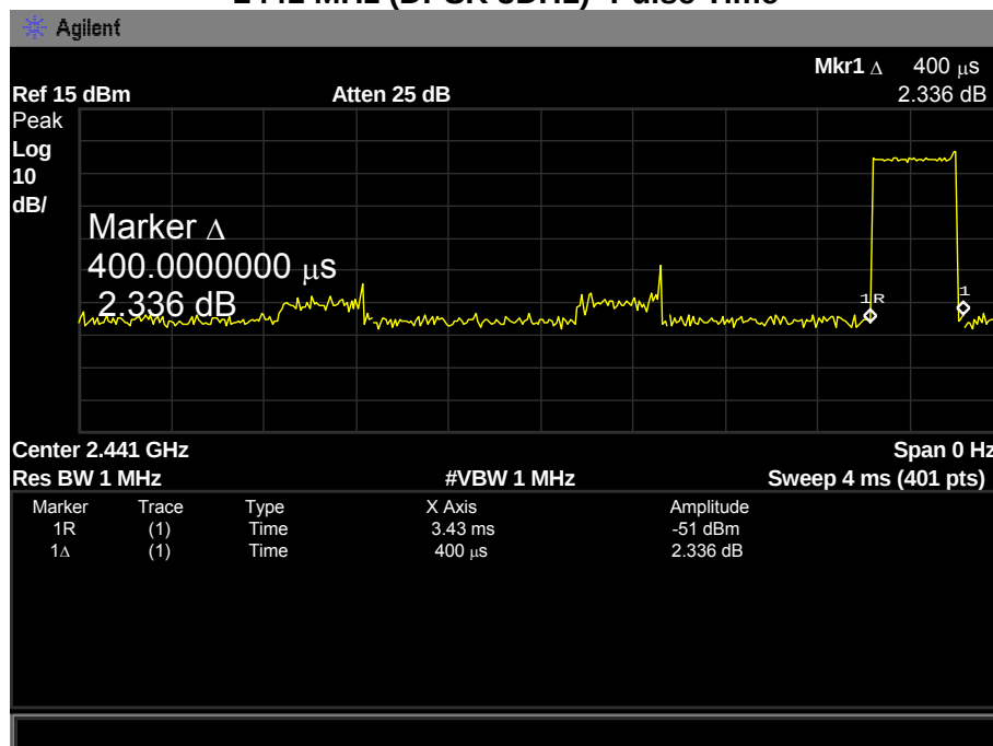
2441 MHz (DPSK 3DH1)- Pulse Time
