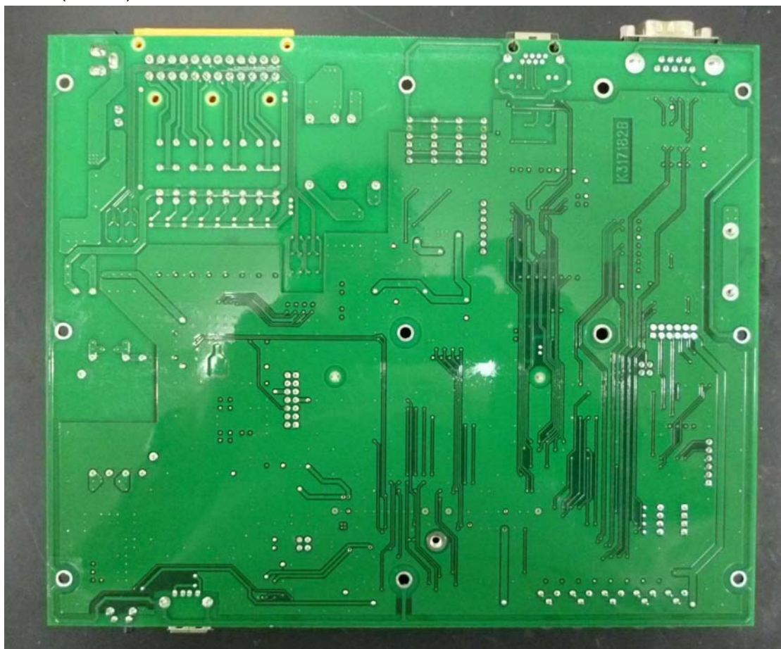
WU-1 Board (Bottom)
