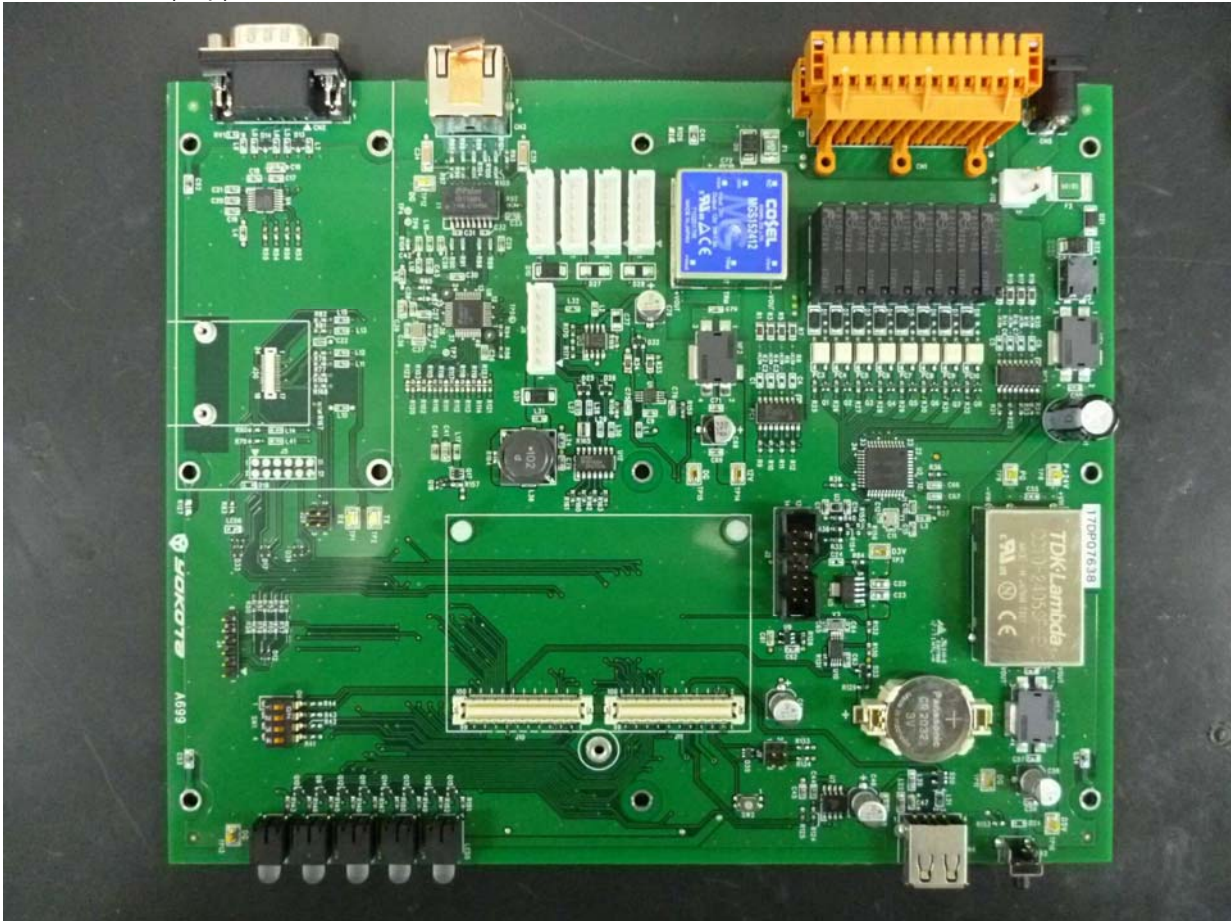
WU-1 Board (Top) CPU Board and Wifi module are no mount.
