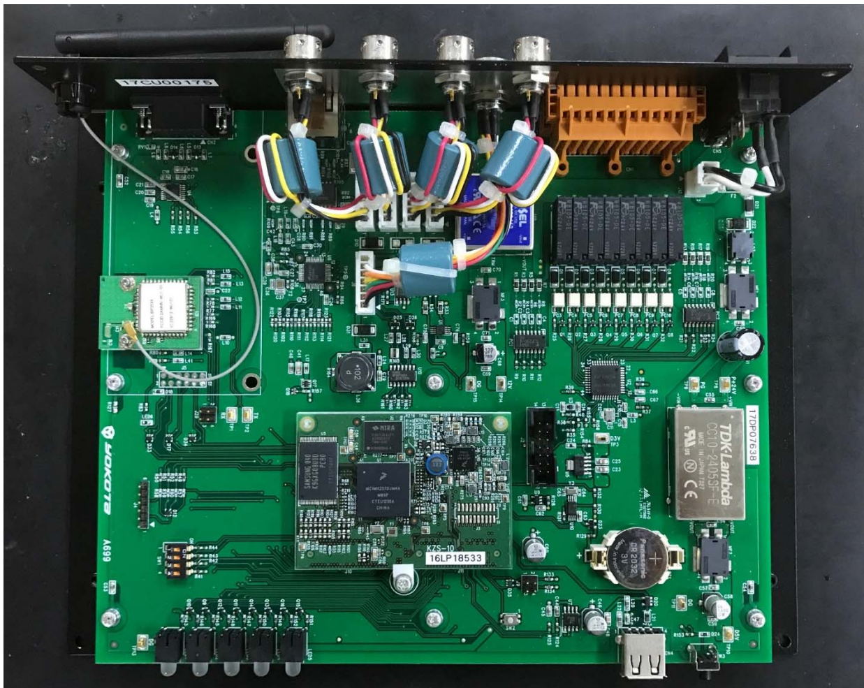
WU-1 Board + CASE
