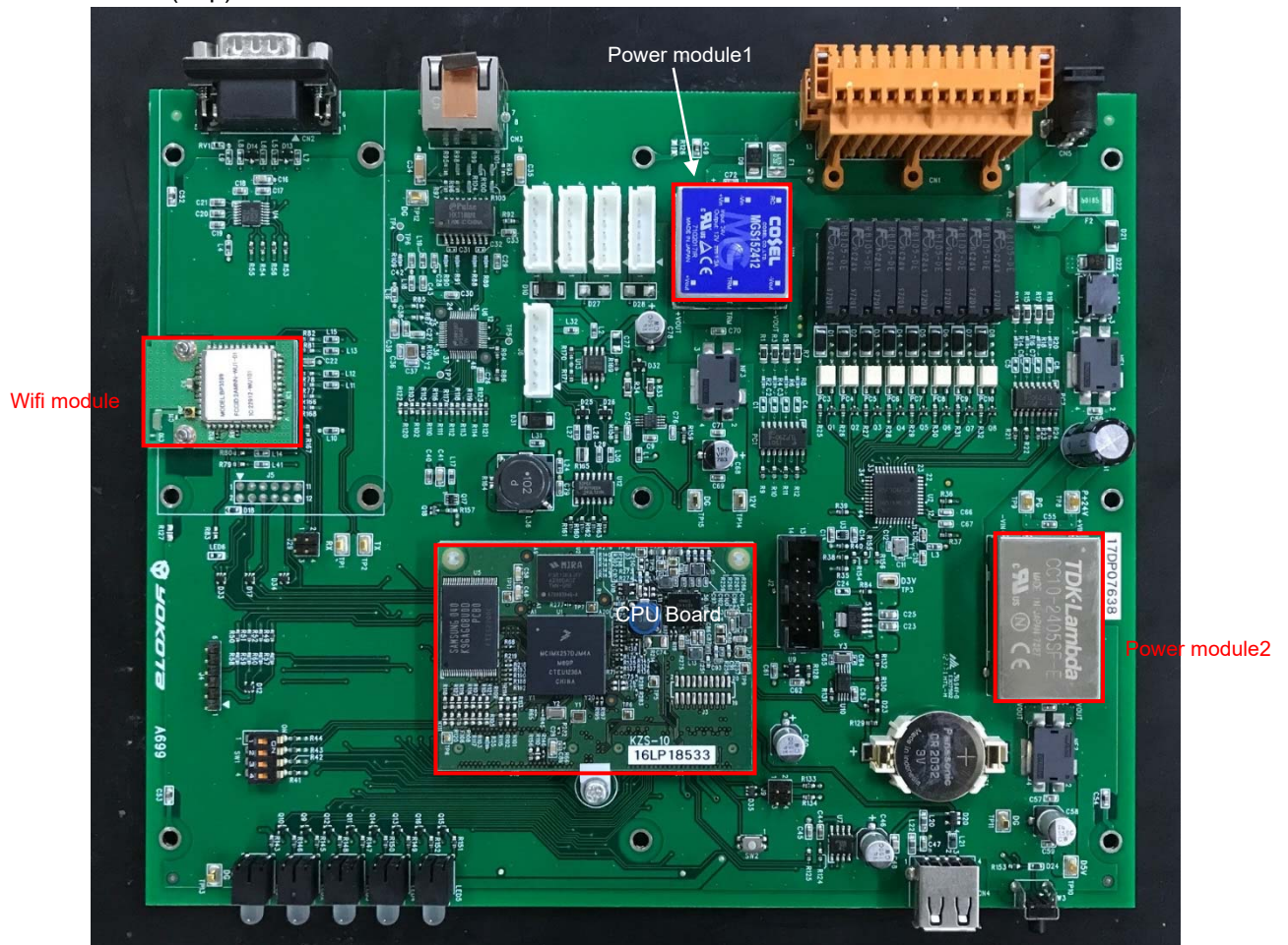
WU-1 Board (Top)
