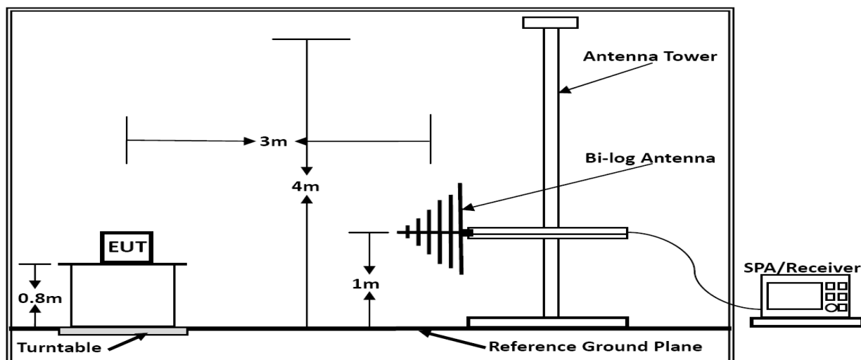
Below 1GHz
