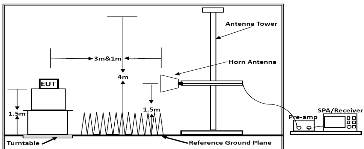
Above 1GHz
