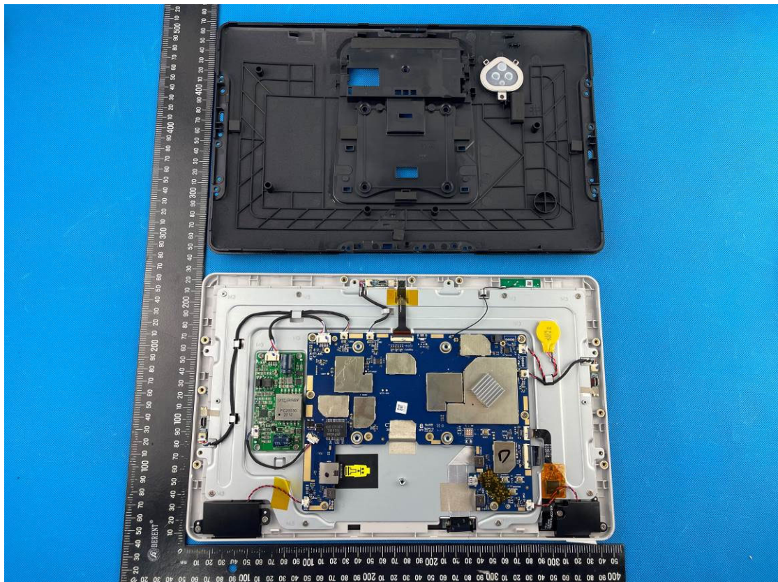
Main LCD panel + Add POE module + Add one speaker ( For TK200&TK300)
