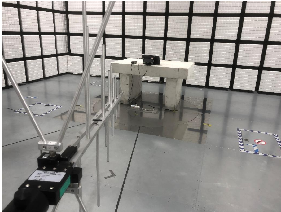
Description: Radiated Emission Test Setup (30MHz -1000MHz)
