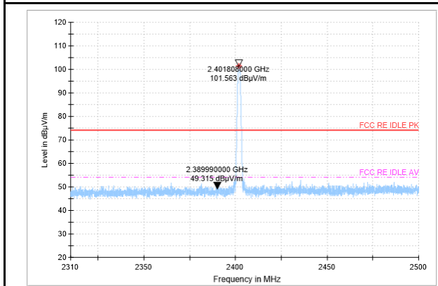
Bandedge (Low): \pi/4 DQPSK, low channel
