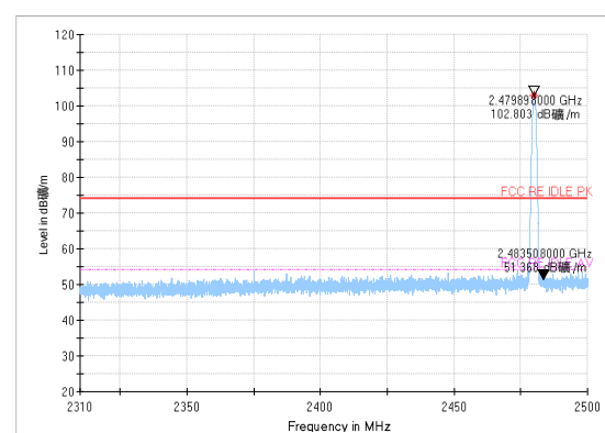
Bandedge:Ch39
