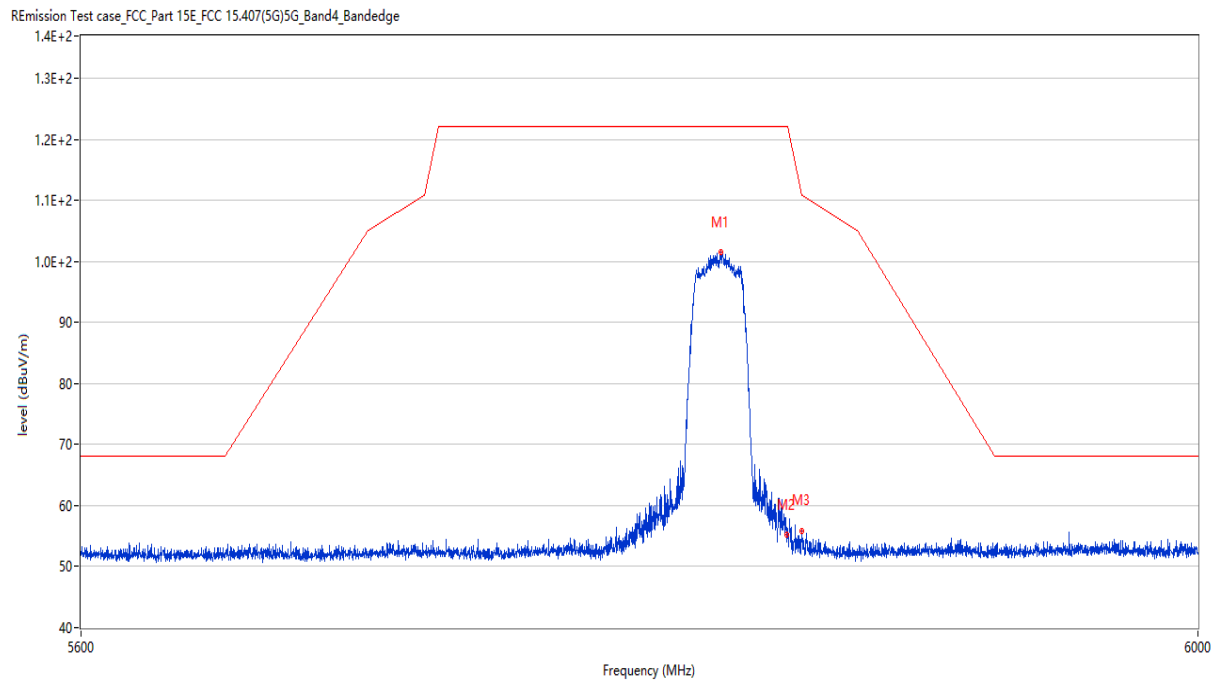
Figure 15: Band Edge (Restricted-band band-edge), 802.11n(HT20), 5825MHz
