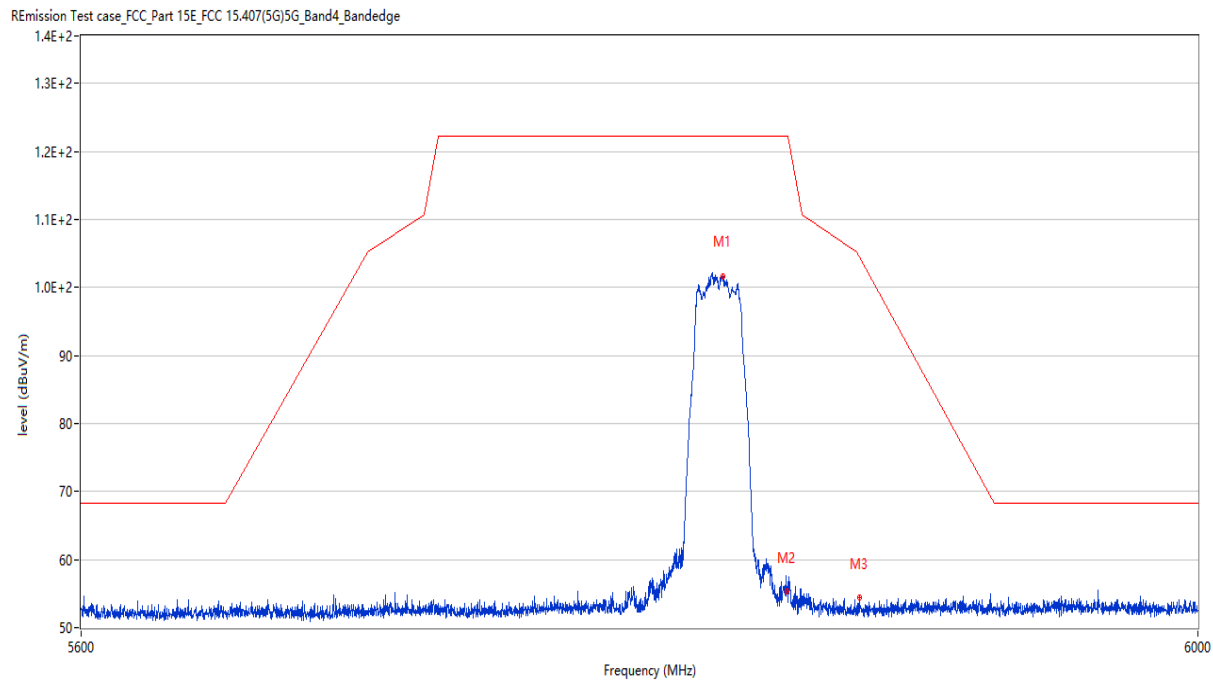
Figure 13: Band Edge (Restricted-band band-edge), 802.11a, 5825MHz
