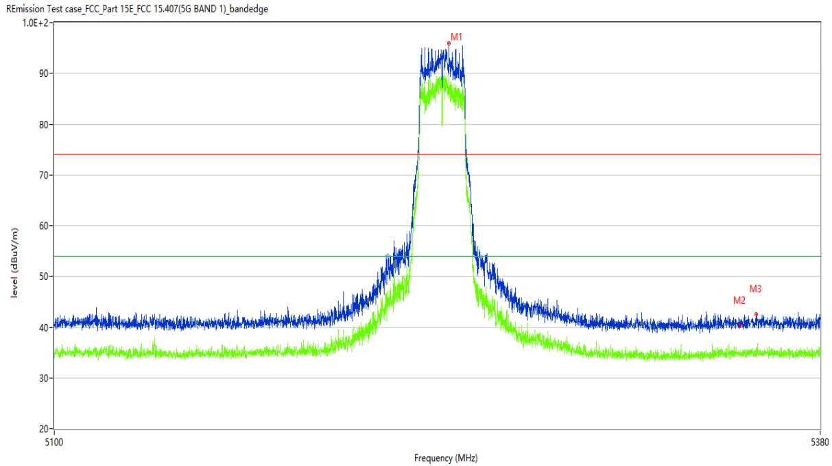
Figure 2: Band Edge (Restricted-band band-edge), 802.11a, 5240MHz
