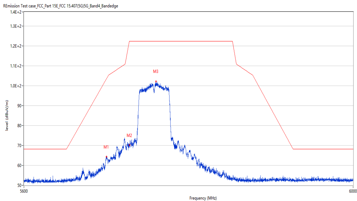
Figure 18: Band Edge (Restricted-band band-edge), 802.11n(HT40), 5755MHz
