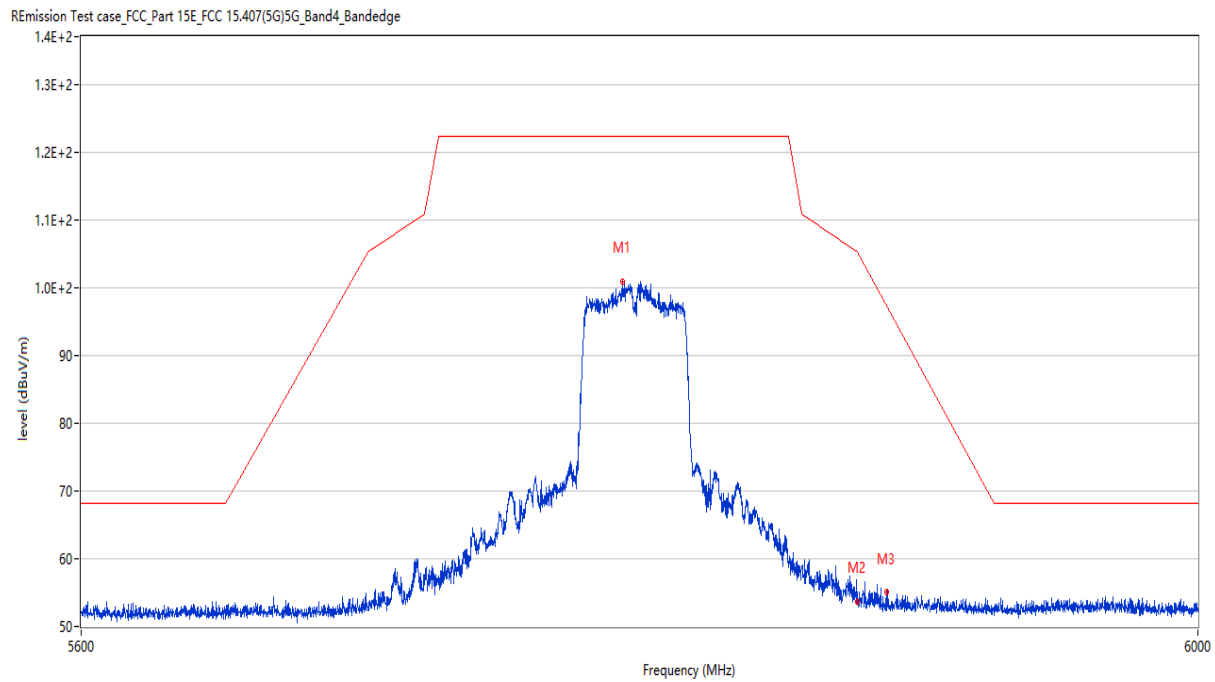
Figure 19: Band Edge (Restricted-band band-edge), 802.11n(HT40), 5795MHz
