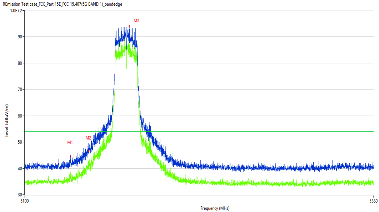
Figure 5: Band Edge (Restricted-band band-edge), 802.11ac(VHT20), 5180MHz
