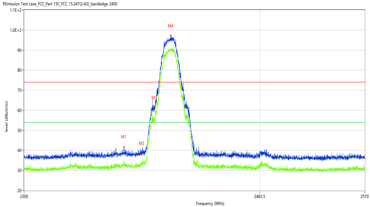
Figure 1: Band Edge (Restricted-band band-edge), 802.11b, 2412MHz
