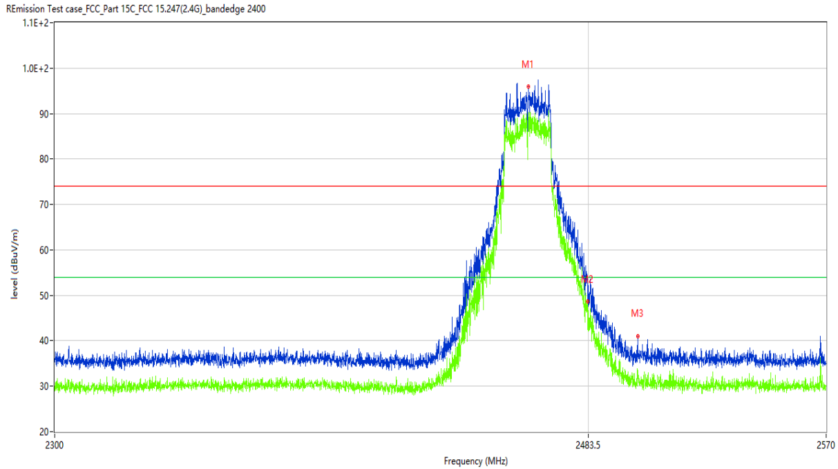
Figure 4: Band Edge (Restricted-band band-edge), 802.11g, 2462MHz
