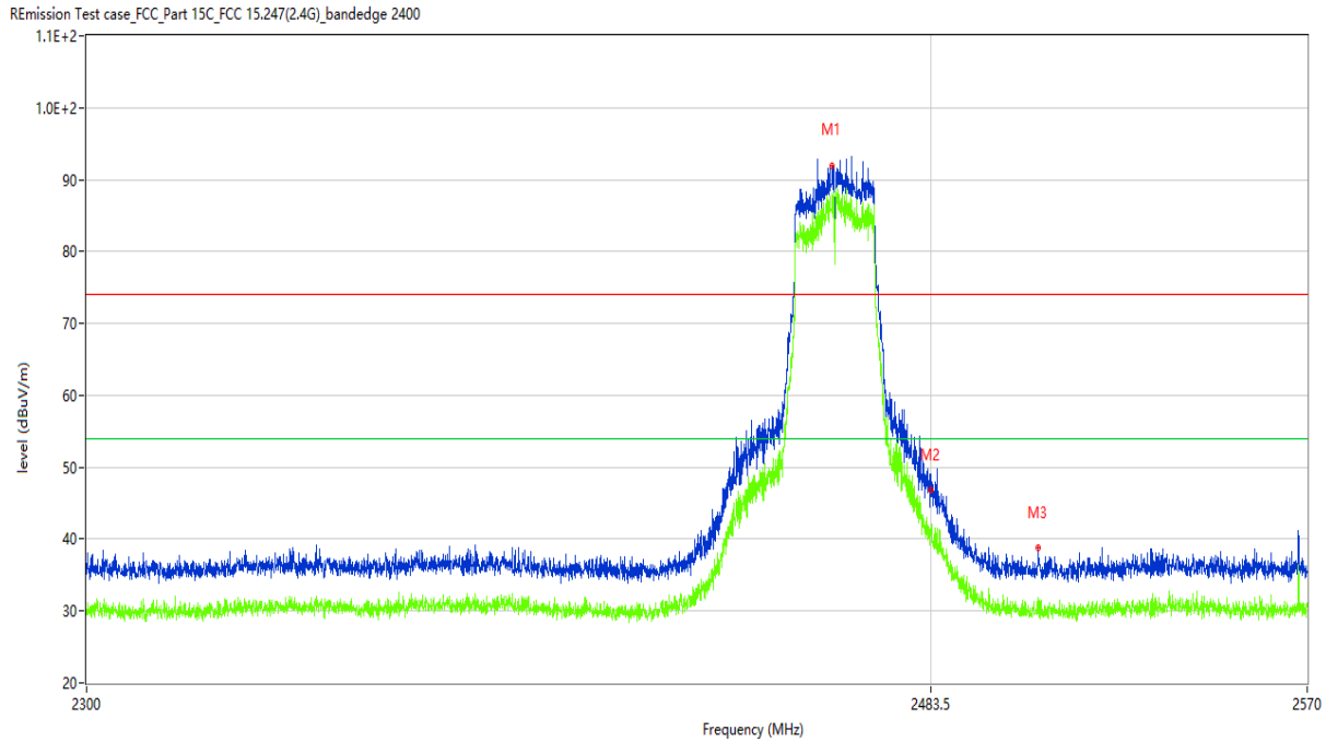
Figure 6: Band Edge (Restricted-band band-edge), 802.11n(HT20), 2462MHz
