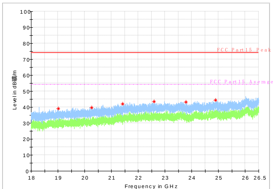
Fig. 68 Radiated Spurious Emission (802.11a, ch36, 18 GHz-26.5 GHz)
