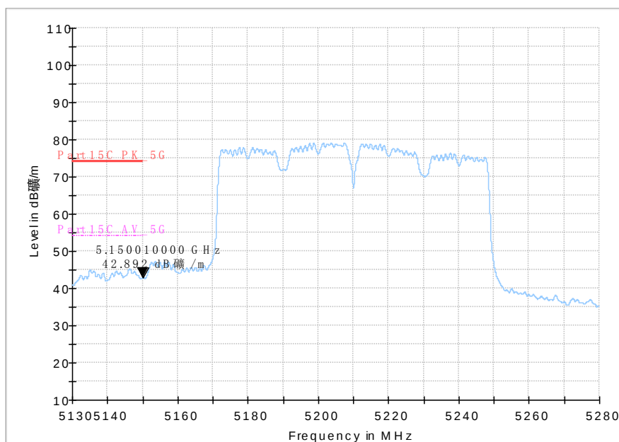
Fig. 64 Band Edges (802.11ac-HT80, 5210MHz)
