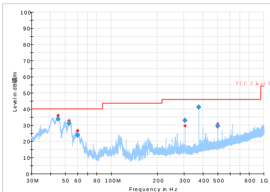
Fig. 70 Radiated Spurious Emission (802.11n-HT20, ch36, 30 MHz-1 GHz)
