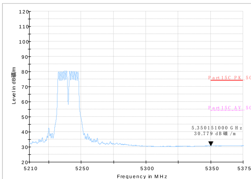
Fig. 61 Band Edges (802.11ac-HT20, 5240MHz)
