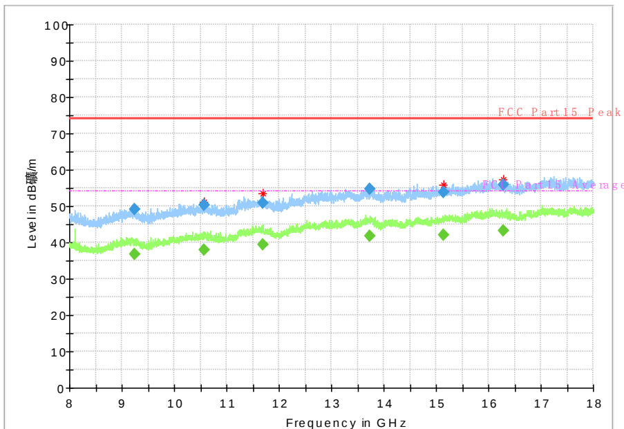
Fig. 72 Radiated Spurious Emission (802.11n-HT20, ch36, 8 GHz-18 GHz)
