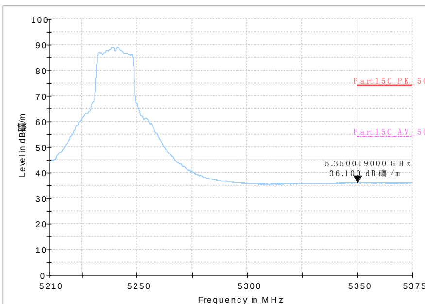
Fig. 55 Band Edges (802.11a, 5240MHz)
