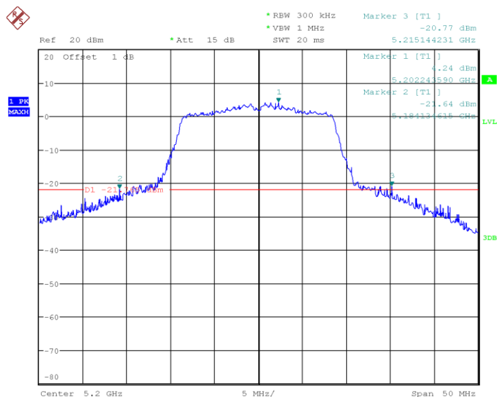
Fig. 23 Occupied 26dB Bandwidth (802.11ac-HT20, 5180MHz)
