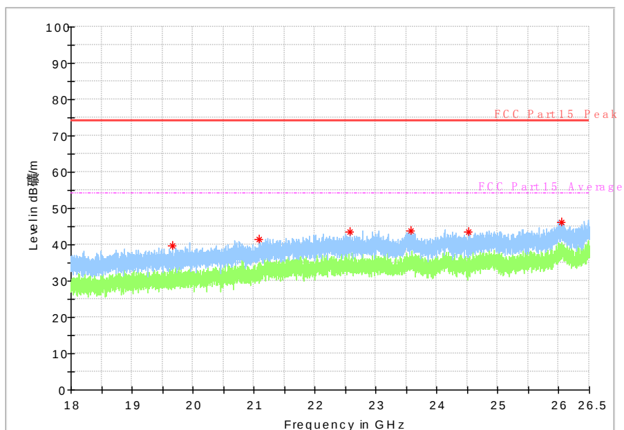
Fig. 83 Radiated Spurious Emission (802.11ac-HT20, Ch36, 18 GHz-26.5 GHz)
