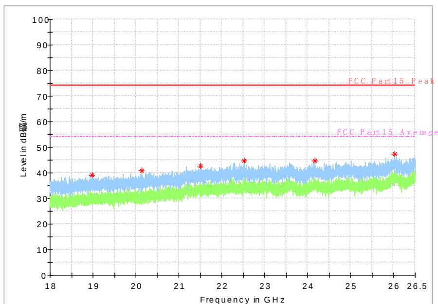
Fig. 88 Radiated Spurious Emission (802.11ac-HT40, Ch38, 18 GHz-26.5 GHz)
