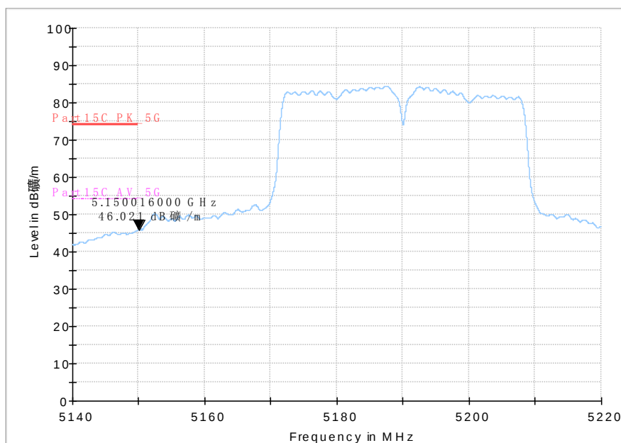
Fig. 62 Band Edges (802.11ac-HT40, 5190MHz)
