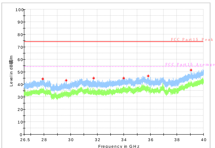
Fig. 84 Radiated emission: 802.11n, (802.11ac-HT20, Ch36, 26.5 GHz - 40 GHz)
