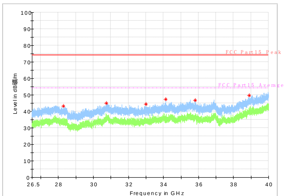
Fig. 74 Radiated Spurious Emission (802.11n-HT20, ch36, 26.5 GHz-40 GHz)
