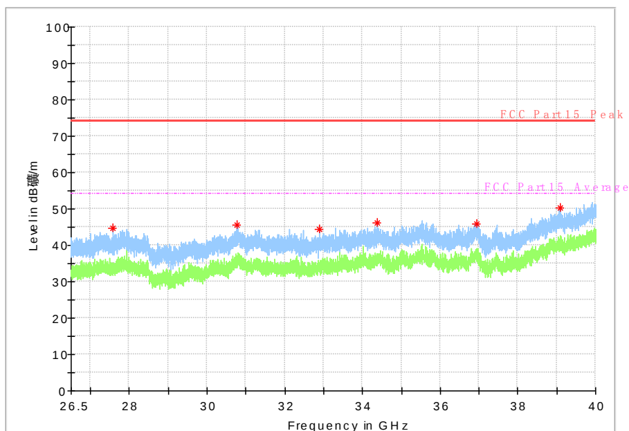
Fig. 69 Radiated Spurious Emission (802.11a, ch36, 26.5 GHz-40 GHz)
