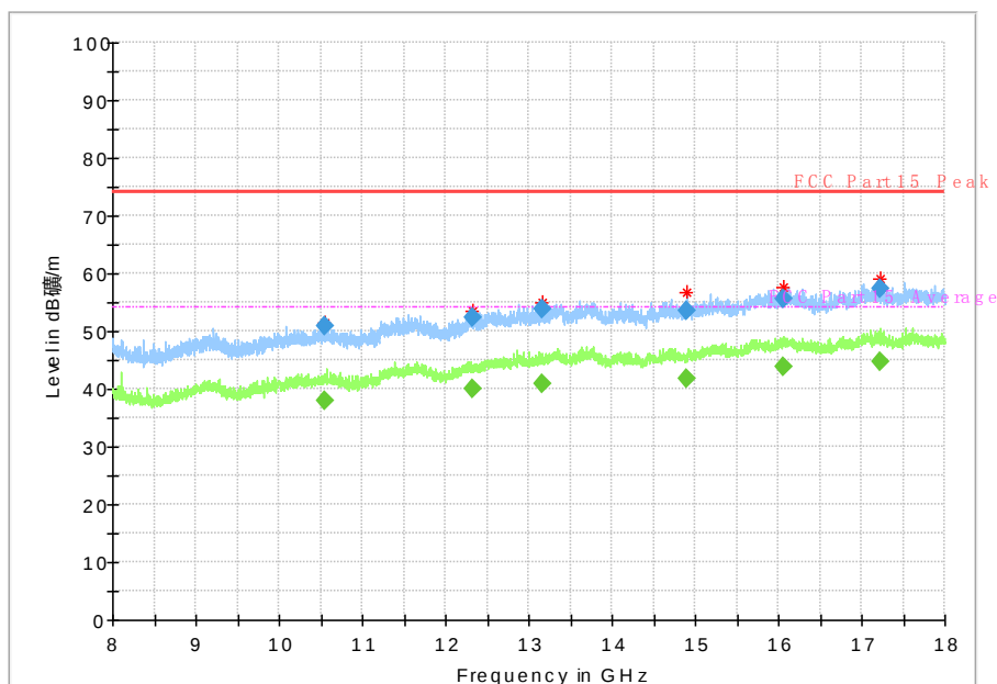
Fig. 67 Radiated Spurious Emission (802.11a, ch36, 8 GHz-18 GHz)
