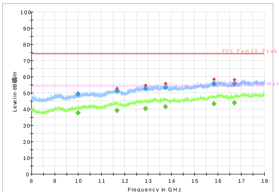
Fig. 87 Radiated Spurious Emission (802.11ac-HT40, Ch38, 8 GHz-18 GHz)
