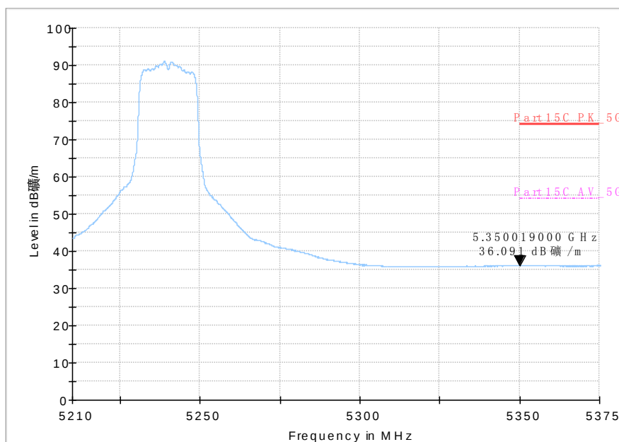
Fig. 57 Band Edges (802.11n-HT20, 5240MHz)
