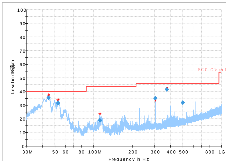
Fig. 80 Radiated Spurious Emission (802.11ac-HT20, Ch36, 30 MHz-1 GHz)
