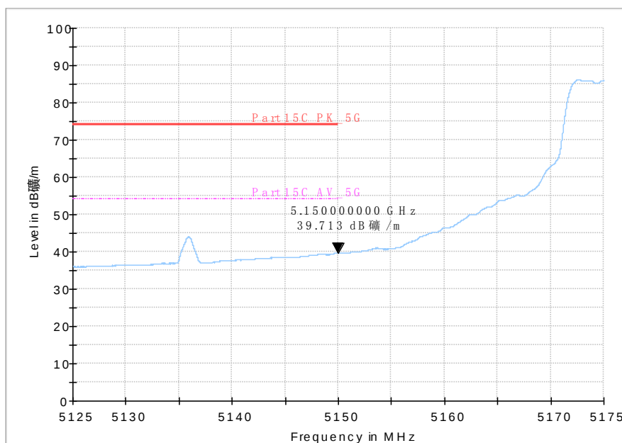
Fig. 54 Band Edges (802.11a, 5180MHz)
