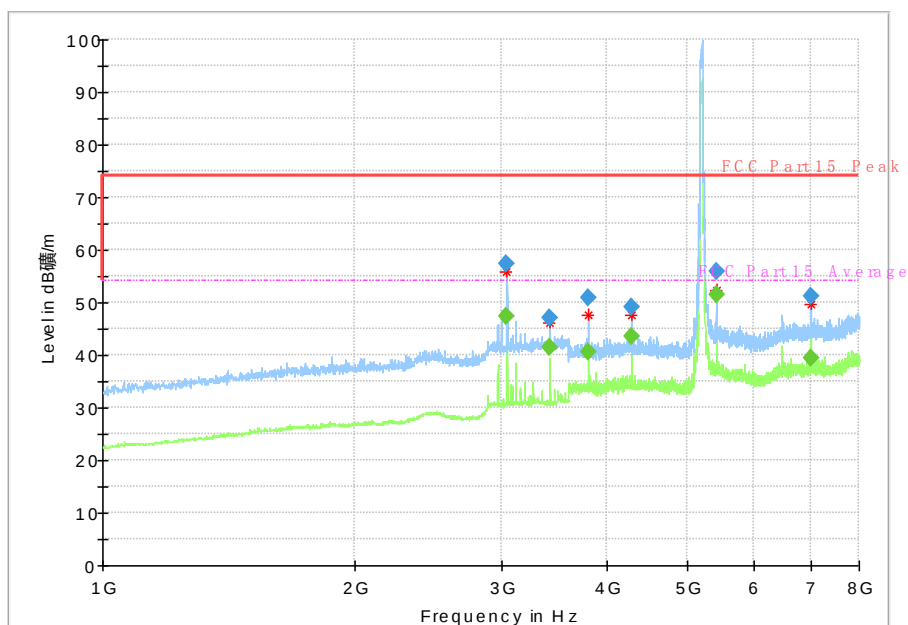
Fig. 86 Radiated Spurious Emission (802.11ac-HT40, Ch38, 1 GHz-8 GHz)
