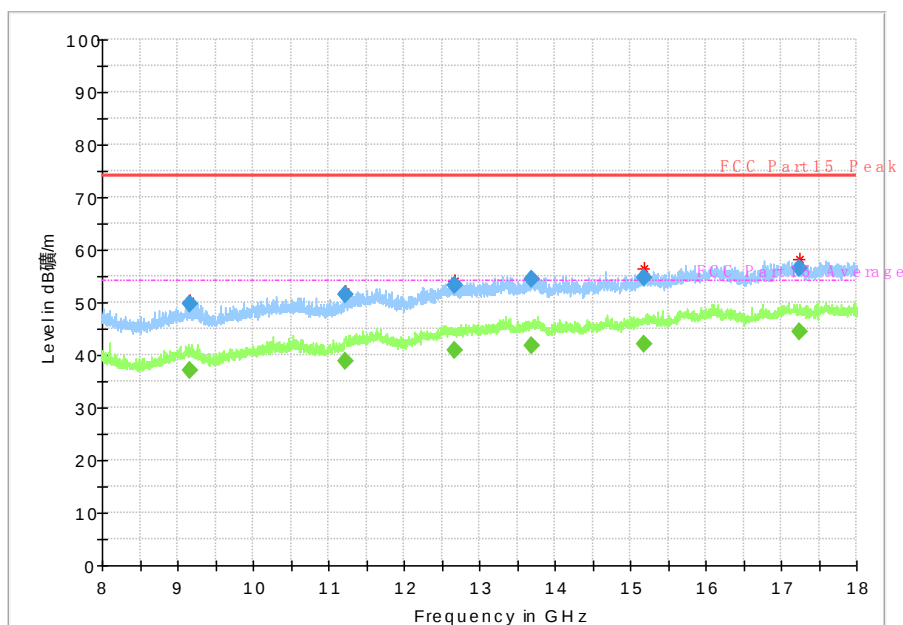
Fig. 82 Radiated Spurious Emission (802.11ac-HT20, Ch36, 8 GHz-18 GHz)
