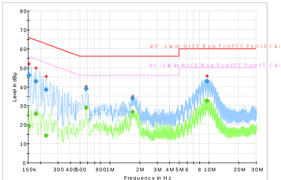
Fig. 96 Conducted Emission(802.11a, TX)
