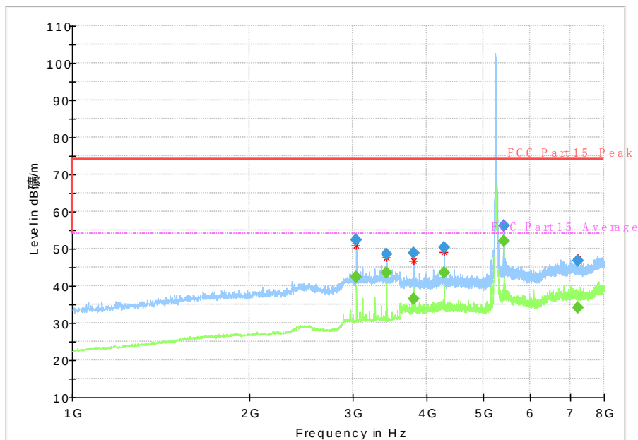
Fig. 71 Radiated Spurious Emission (802.11n-HT20, ch36, 1 GHz-8 GHz)
