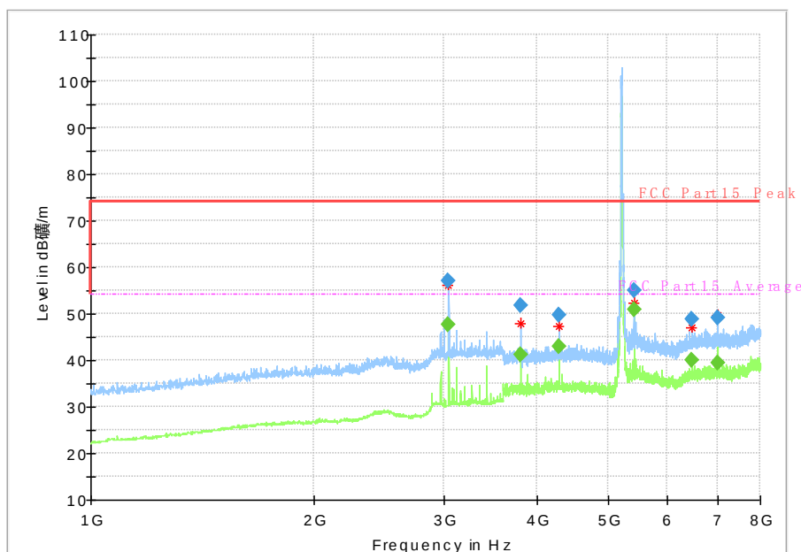
Fig. 66 Radiated Spurious Emission (802.11a, ch36, 1 GHz-8 GHz)
