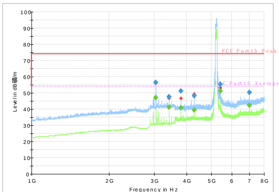
Fig. 91 Radiated Spurious Emission (802.11ac-HT80, Ch42, 1 GHz-8 GHz)
