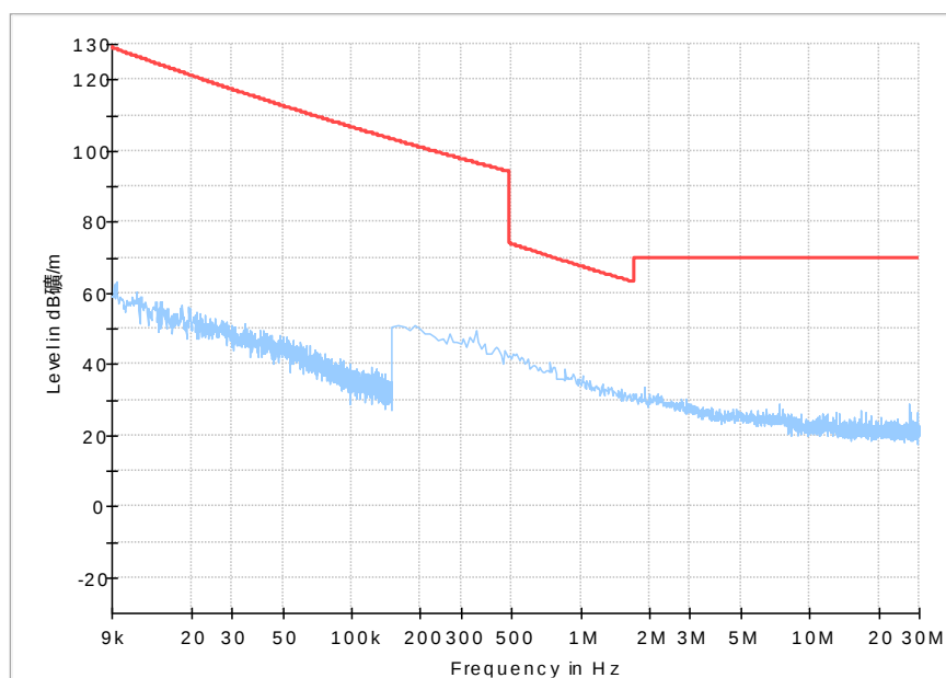
Fig. 95 Radiated Spurious Emission (9kHz-30MHz)
