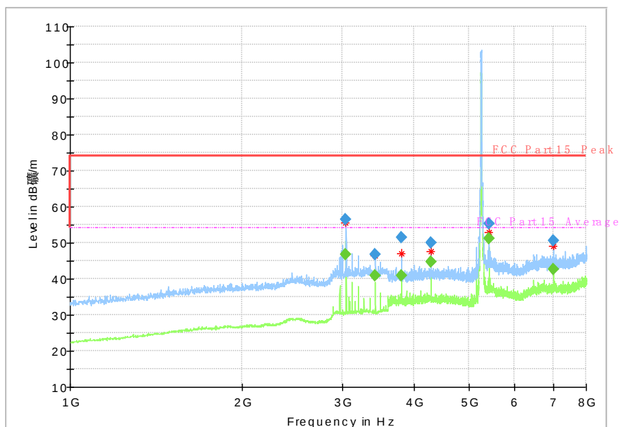
Fig. 81 Radiated Spurious Emission (802.11ac-HT20, Ch36, 1 GHz-8 GHz)
