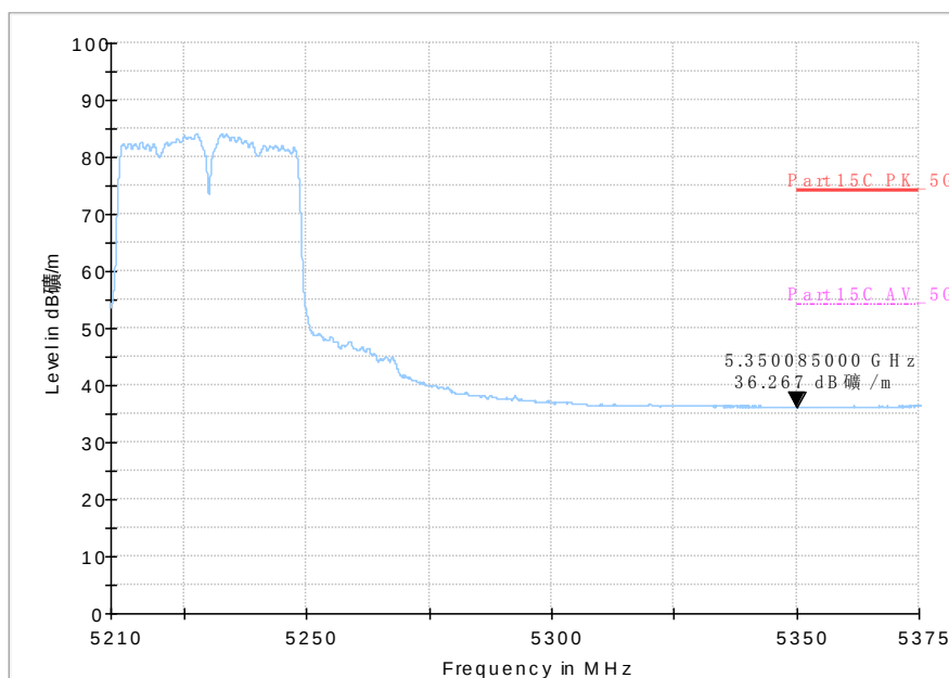
Fig. 59 Band Edges (802.11n-HT40, 5230MHz)
