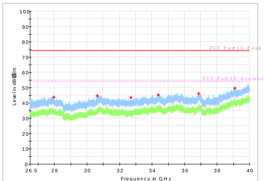
Fig. 89 Radiated emission: 802.11n, (802.11ac-HT40, Ch38, 26.5 GHz - 40 GHz)
