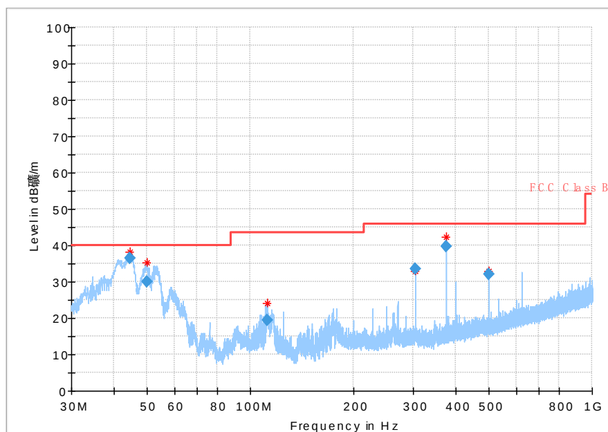
Fig. 90 Radiated Spurious Emission (802.11ac-HT80, Ch42, 30 MHz-1 GHz)
