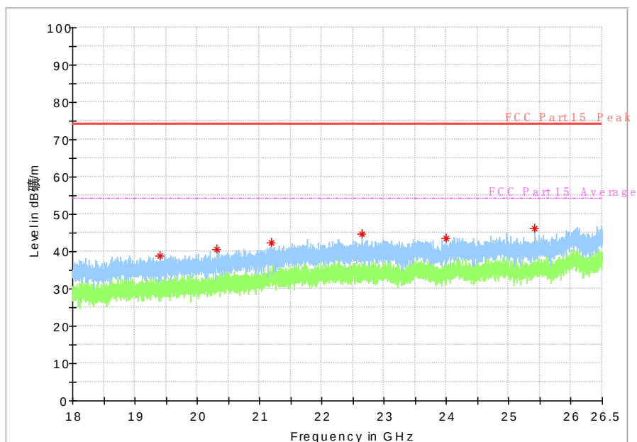
Fig. 73 Radiated Spurious Emission (802.11n-HT20, ch36, 18 GHz-26.5 GHz)
