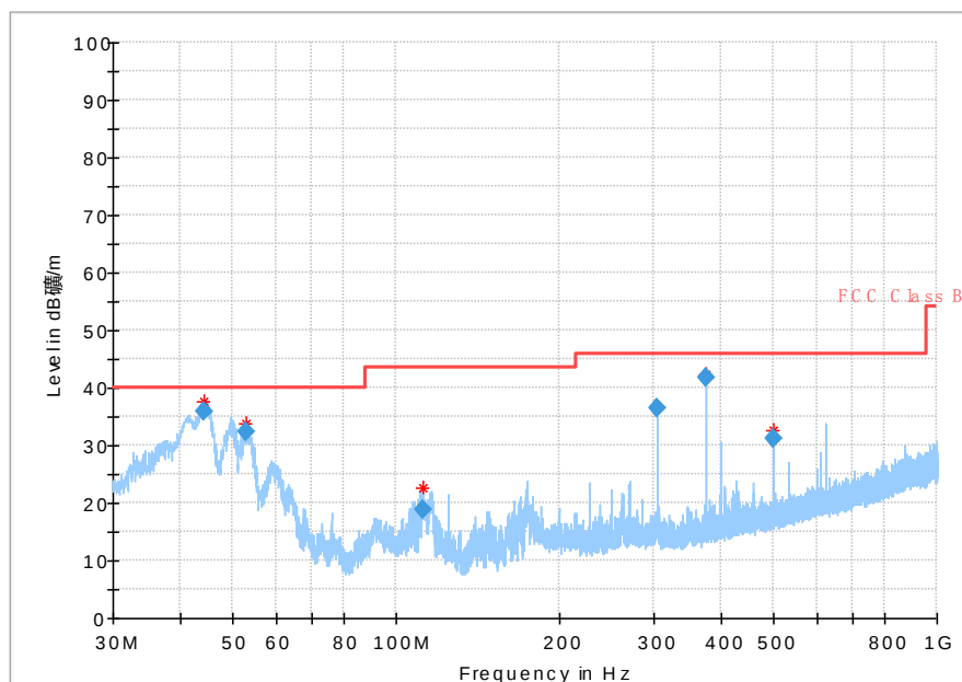
Fig. 85 Radiated Spurious Emission (802.11ac-HT40, Ch38, 30 MHz-1 GHz)
