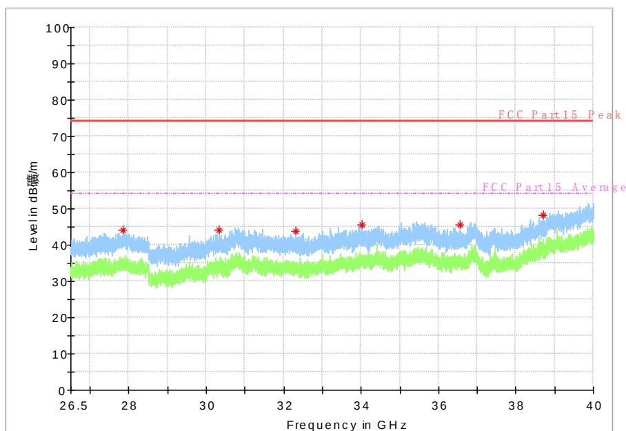
Fig. 94 Radiated emission: 802.11n, (802.11ac-HT80, Ch42, 26.5 GHz - 40 GHz)
