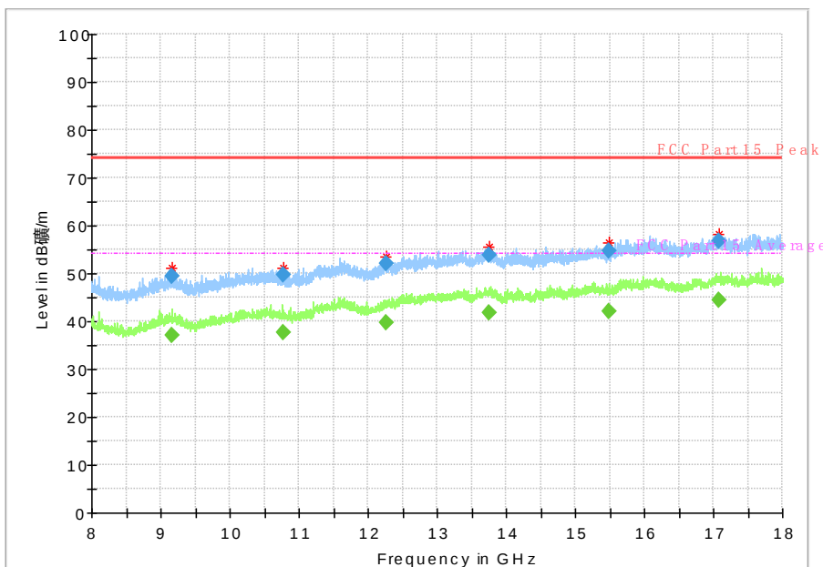
Fig. 92 Radiated Spurious Emission (802.11ac-HT80, Ch42, 8 GHz-18 GHz)
