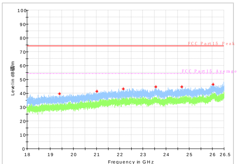
Fig. 93 Radiated Spurious Emission (802.11ac-HT80, Ch42, 18 GHz-26.5 GHz)
