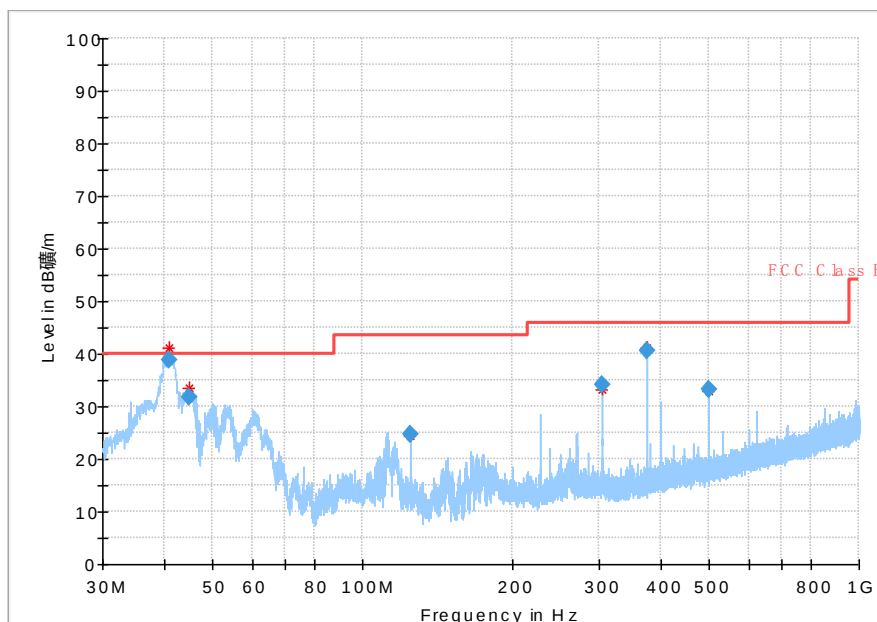
Fig. 65 Radiated Spurious Emission (802.11a, ch36, 30 MHz-1 GHz)
