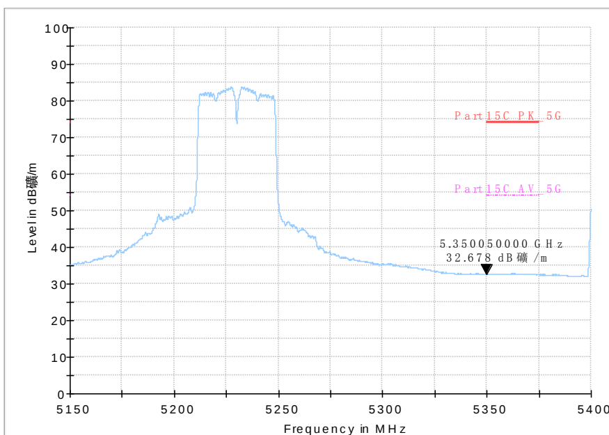
Fig. 63 Band Edges (802.11ac-HT40, 5230MHz)
