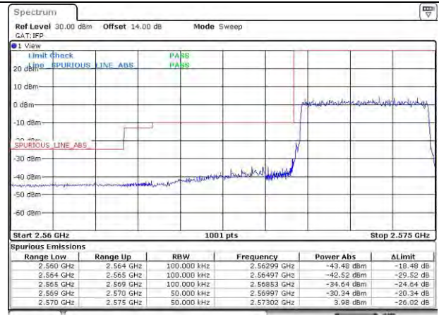
LTE Band 38_2572.5 MHz_5M_QPSK_FRB
