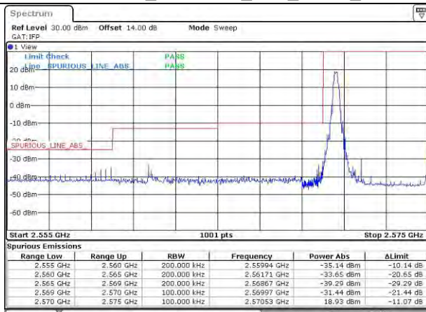
LTE Band 38_2575 MHz_10M_QPSK_1RB
