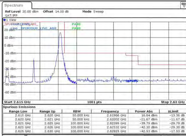
LTE Band 38_2617.5 MHz_5M_QPSK_1RB
