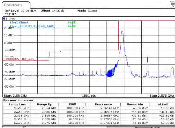
LTE Band 38_2572.5 MHz_5M_QPSK_1RB
