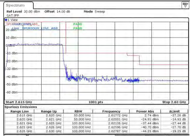
LTE Band 38_2617.5 MHz_3M_QPSK_FRB
