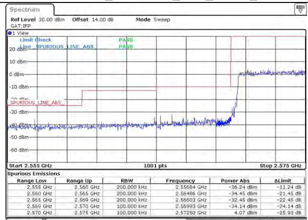
LTE Band 38_2575 MHz_10M_QPSK_FRB
