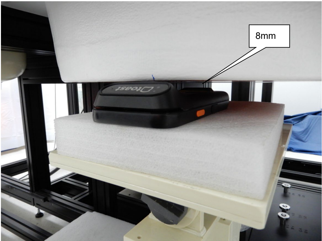
EUT Back_8mm (WWAN)
