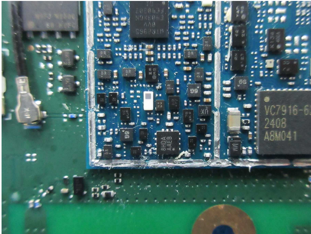
(68) EUT Photo (LTE Main Antenna)
