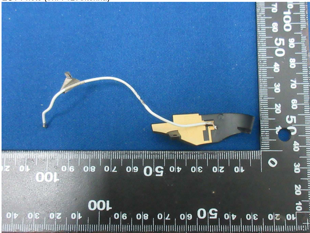
(26) EUT Photo (WiFi 1L Antenna)
