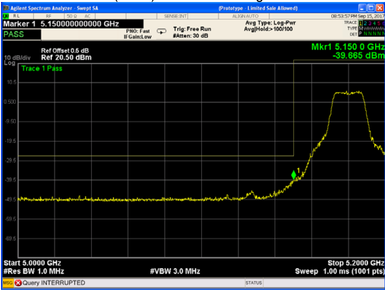
802.11a(HT20) U-NII-1 Band edge-left side
