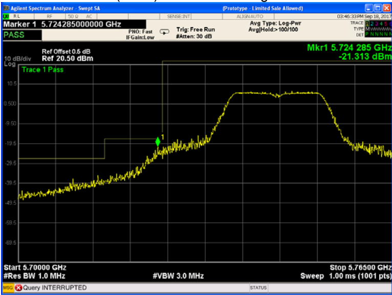
802.11a(HT20) U-NII-3 Band edge-left side
