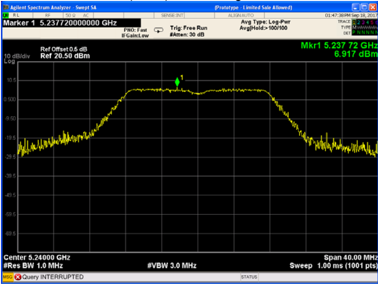
802.11a(HT20) U-NII-1 High channel
