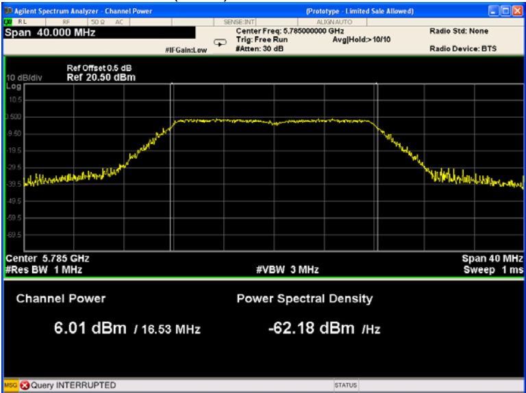
802.11a(HT20) U-NII-3 Middle channel
