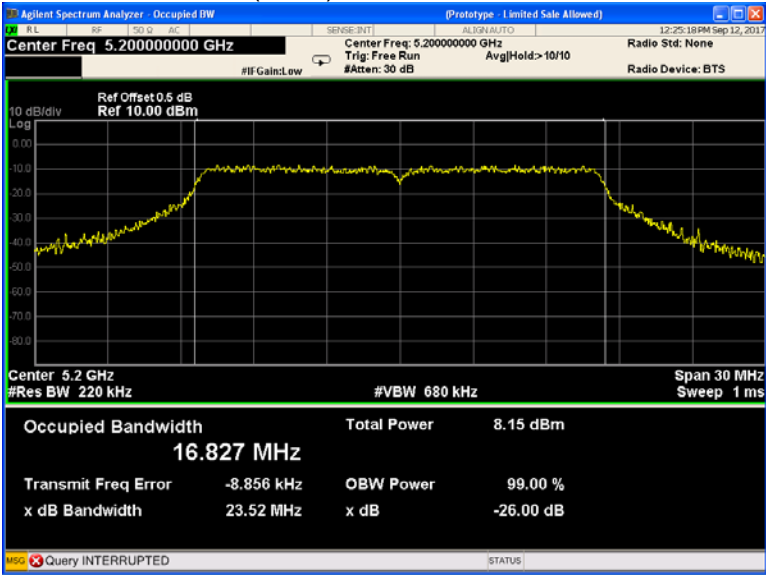
802.11a(HT20) U-NII-1 Middle channel
