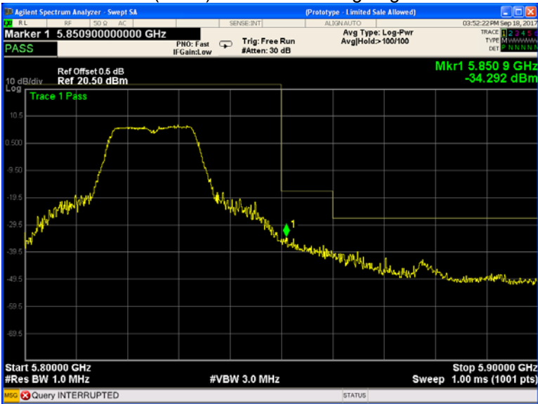
802.11a(HT20) U-NII-3 Band edge-right side
