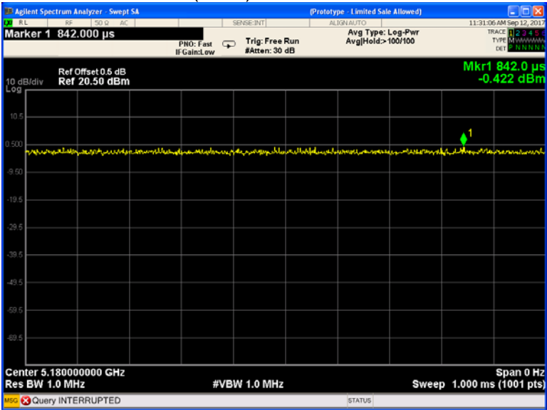
802.11a(HT20) U-NII-1 Low channel
