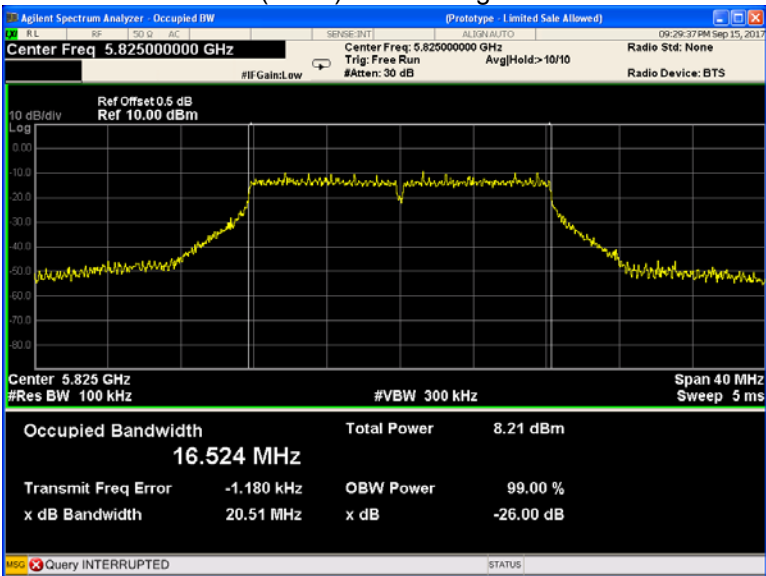
802.11a(HT20) U-NII-3 High channel
