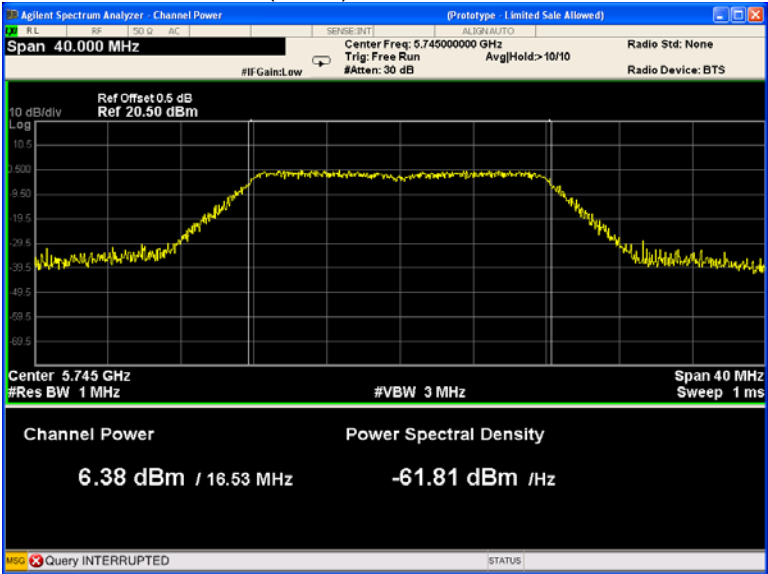
802.11a(HT20) U-NII-3 Low channel
