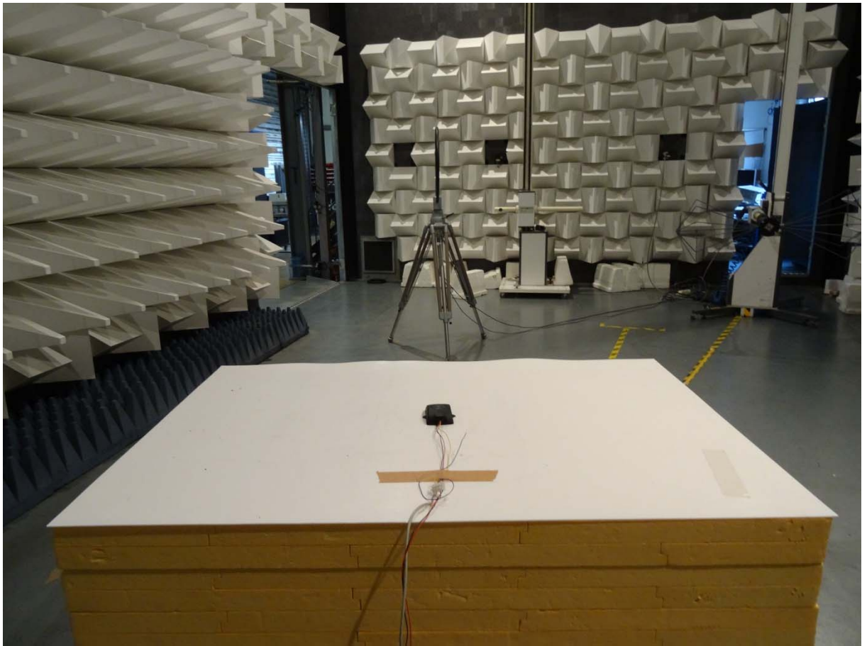
Radiated < 30MHz
