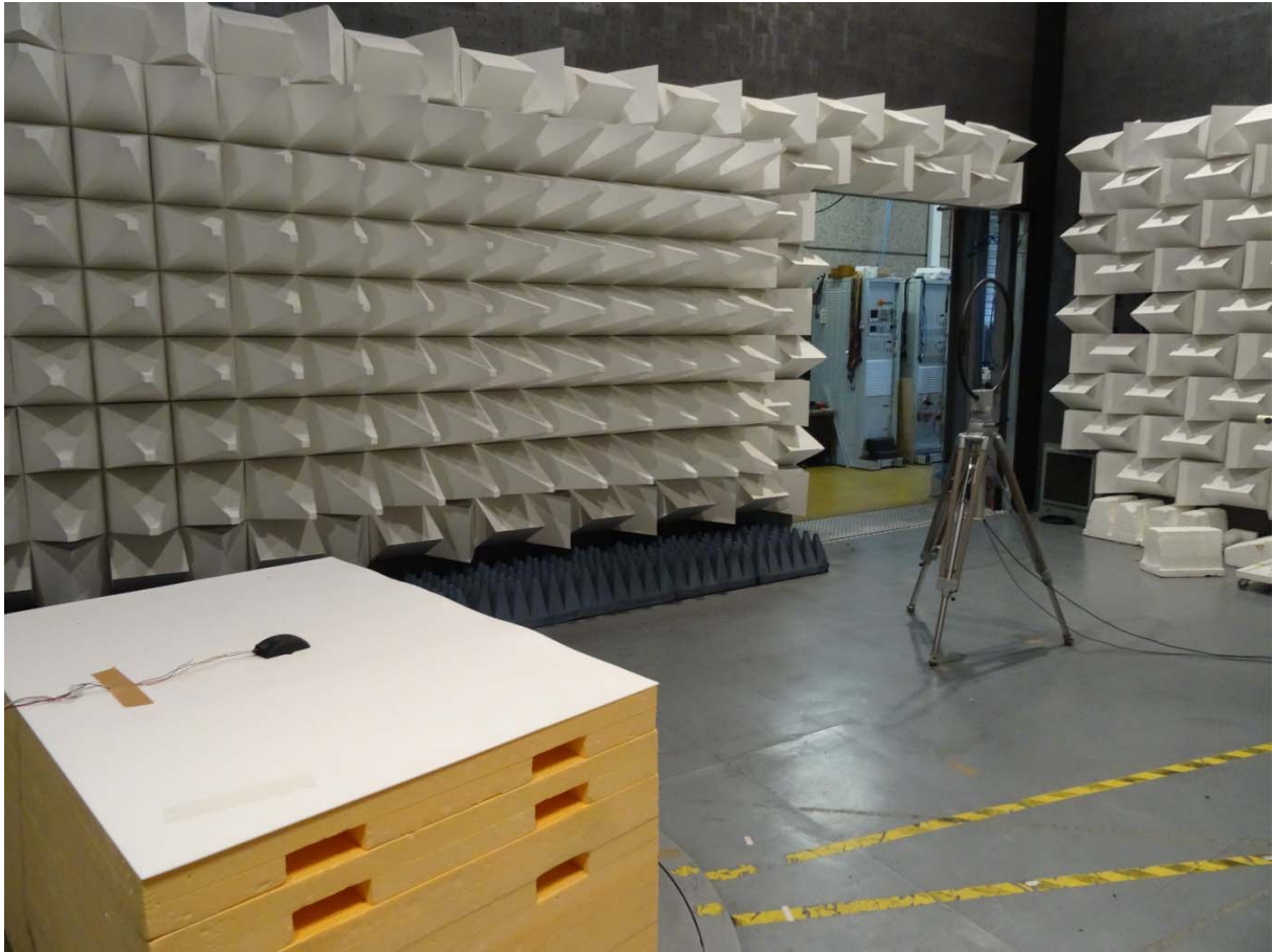
Radiated < 30MHz
