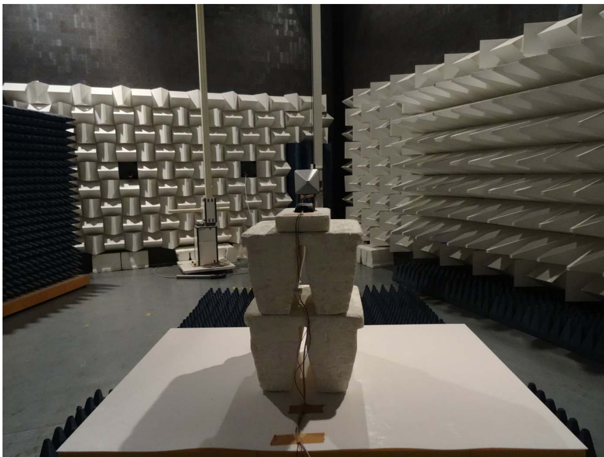
Radiated emission 1GHz - 10 GHz
