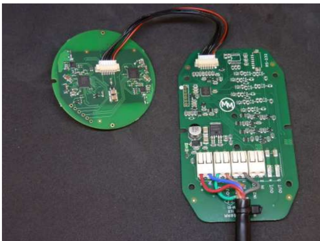
Internal photos
