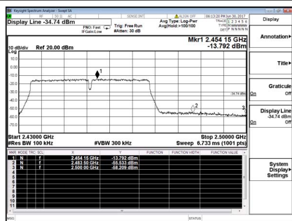
802.11n(HT40)-High channel
