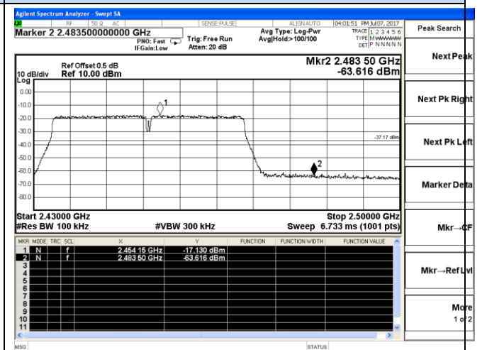
802.11n(HT40)-High channel
