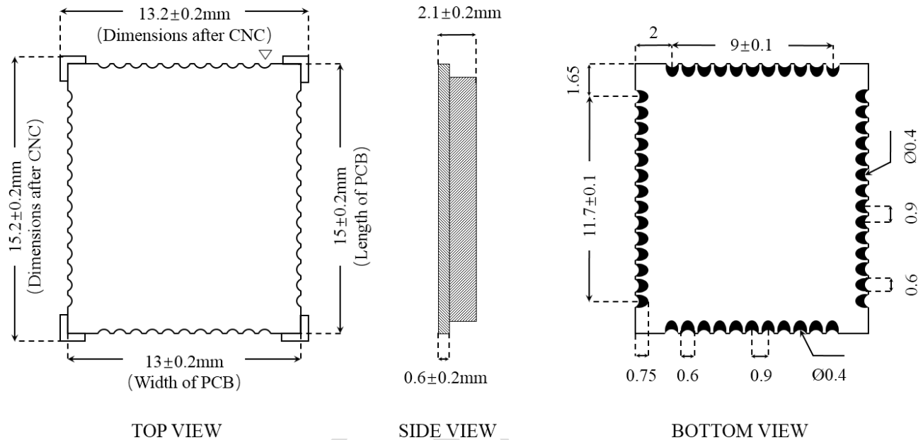
FIG 6 EWN-8822CSS3DA Module Dimension
