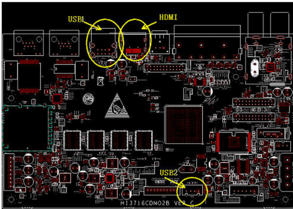
Fig 11 HDIM and USB interference
