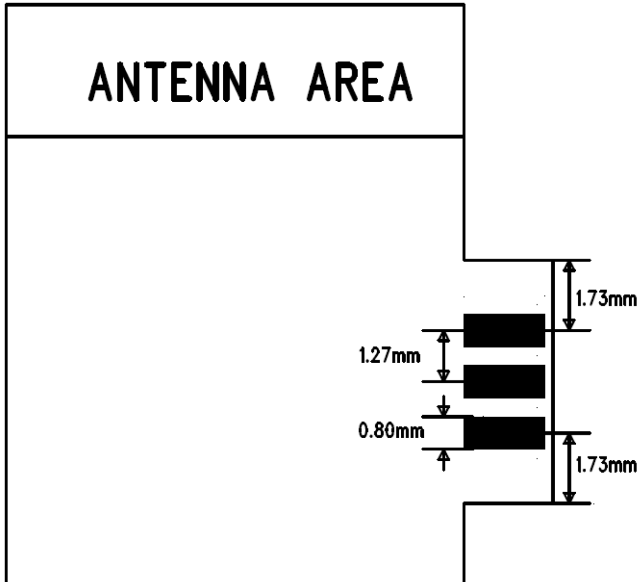
Fig 3 EWN-8258FAT1HA Bottom View Module Size
